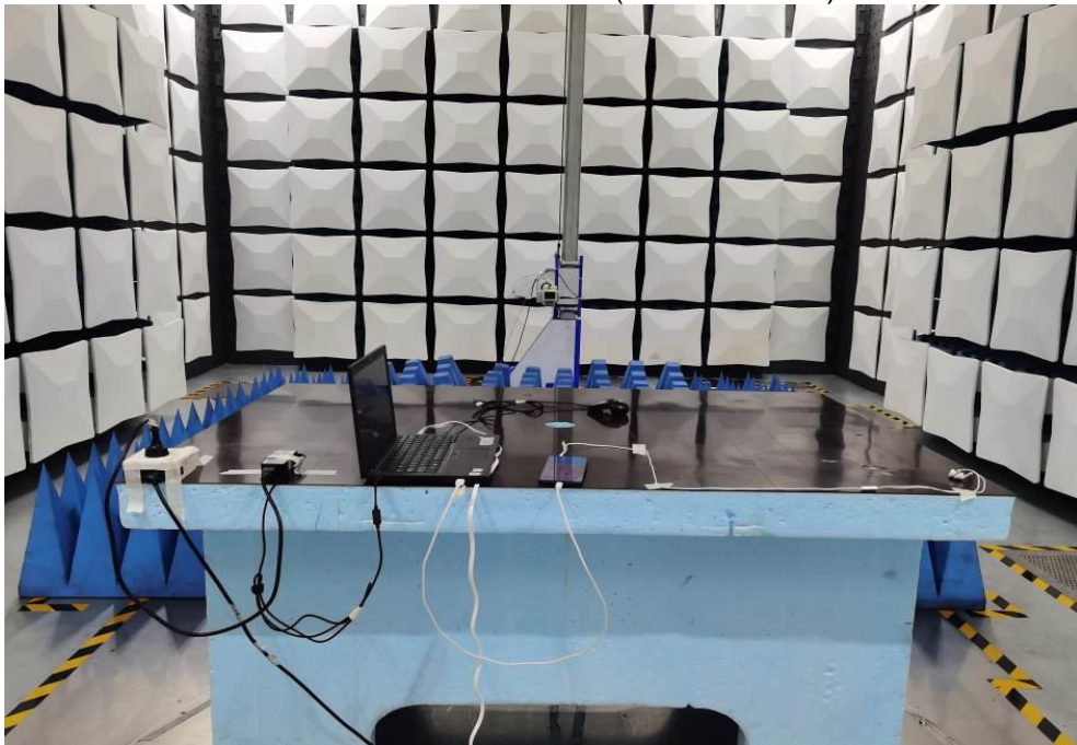
Radiated Disturbance Emissions (18GHz to 40GHz)
