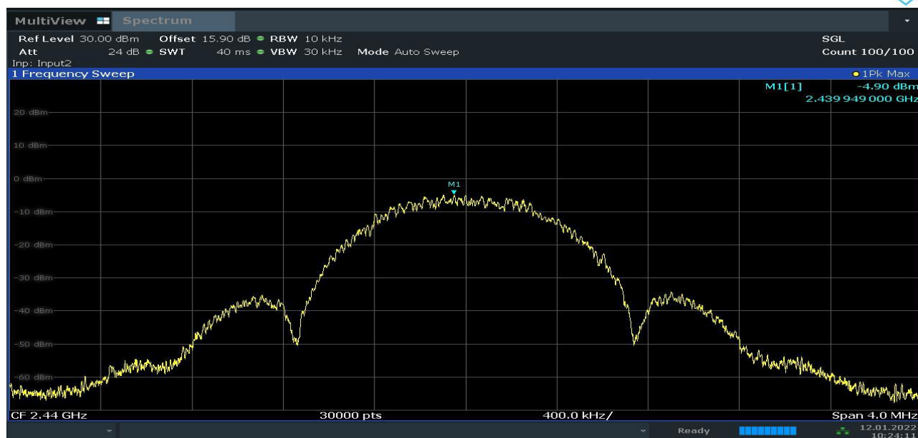
BLE_TM1_Ant1_2440
