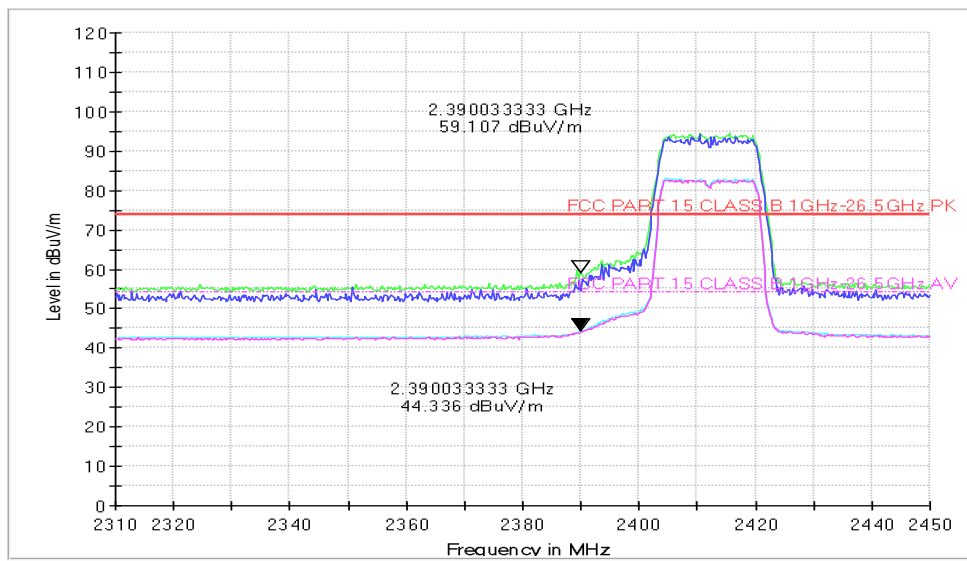
CH_2412 (Band Edge)
