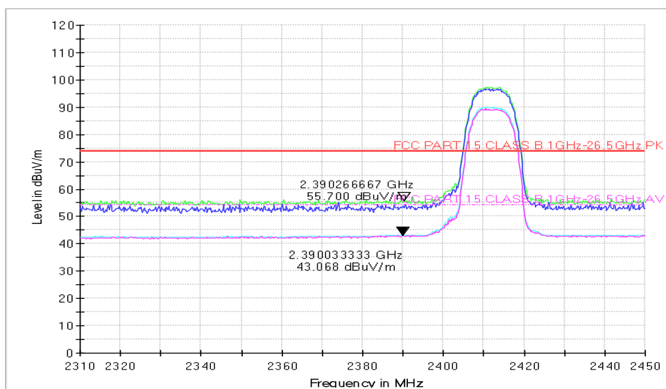
CH_2412 (Band Edge)
