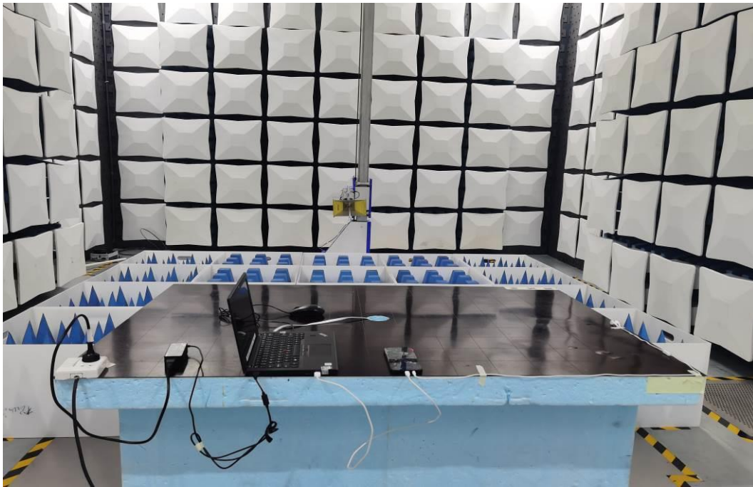
Radiated Disturbance Emission (1GHz to18GHz)
