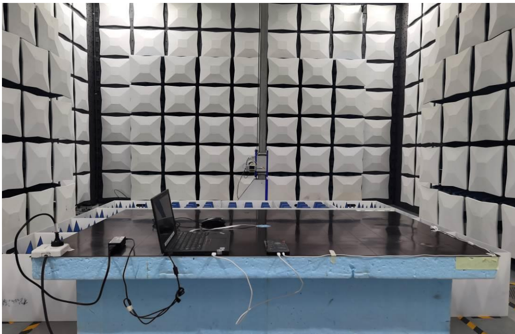
Radiated Disturbance Emission (18GHz to 40GHz)
