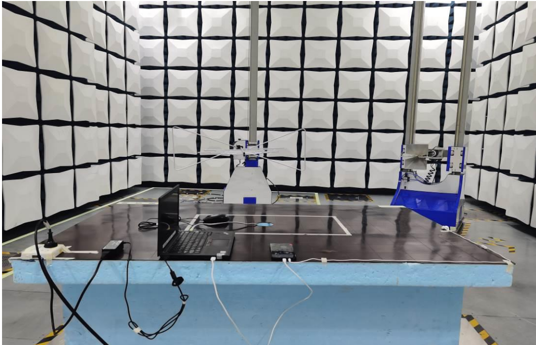
Radiated Disturbance Emission (below 1GHz)
