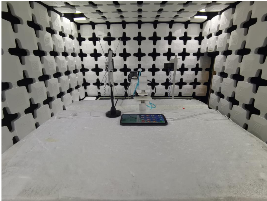
Radiated Spurious Emission (30 MHz to 3 GHz)
