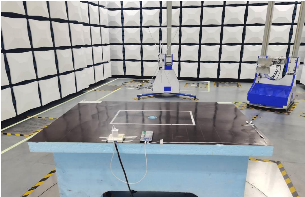
Radiated Spurious Emission (30MHz-1GHz)
