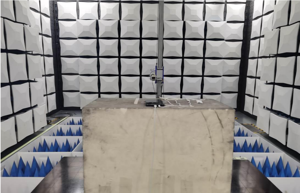
Radiated Spurious Emission (above 18GHz)
