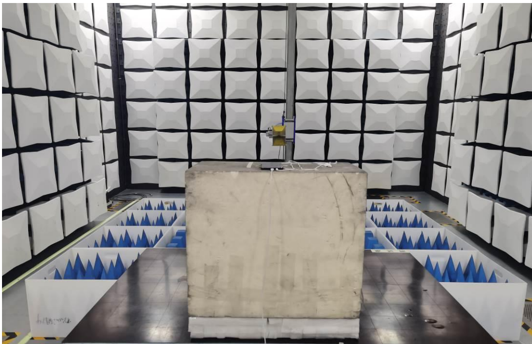
Radiated Spurious Emission (1GHz-18GHz)
