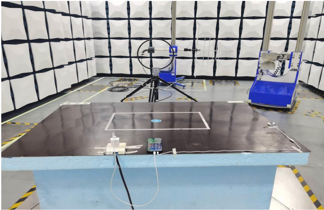
Radiated Spurious Emission (9K-30MHz)
