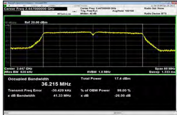
802.11n(HT40), Carrier frequency (MHz):2447
