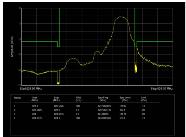
LTE Band 26 64QAM 1.4MHz CH-High 100%RB
