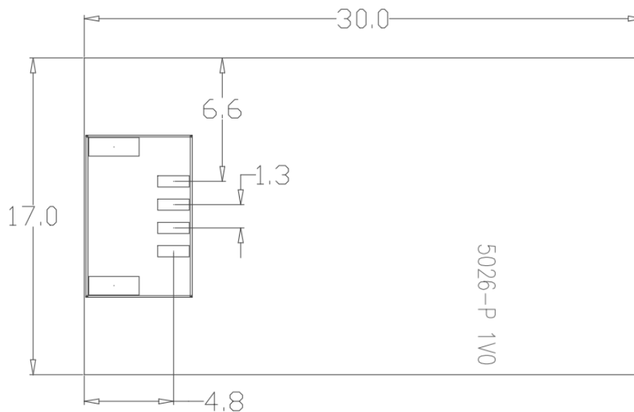
Fig 3: BL5026-P Dimensions
