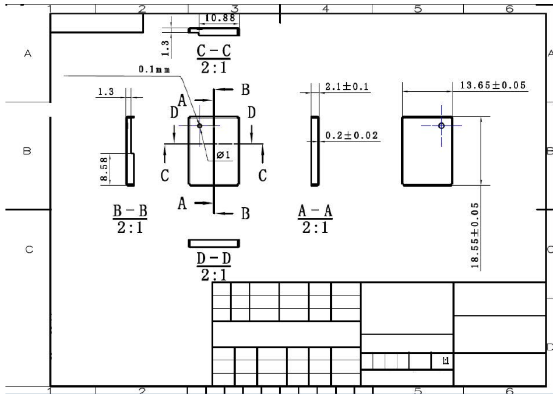
Fig 6: BL5026-P Dimensions of shielding case
