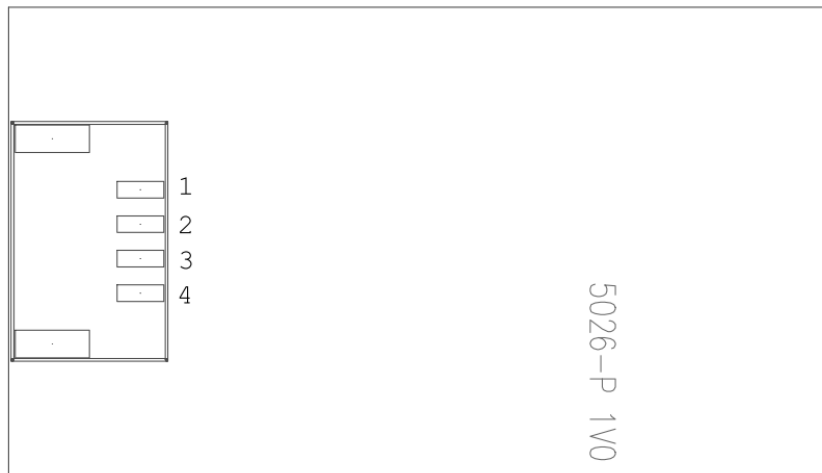
Fig 1:BL5026-P pin sequence(TOP VIEW)
