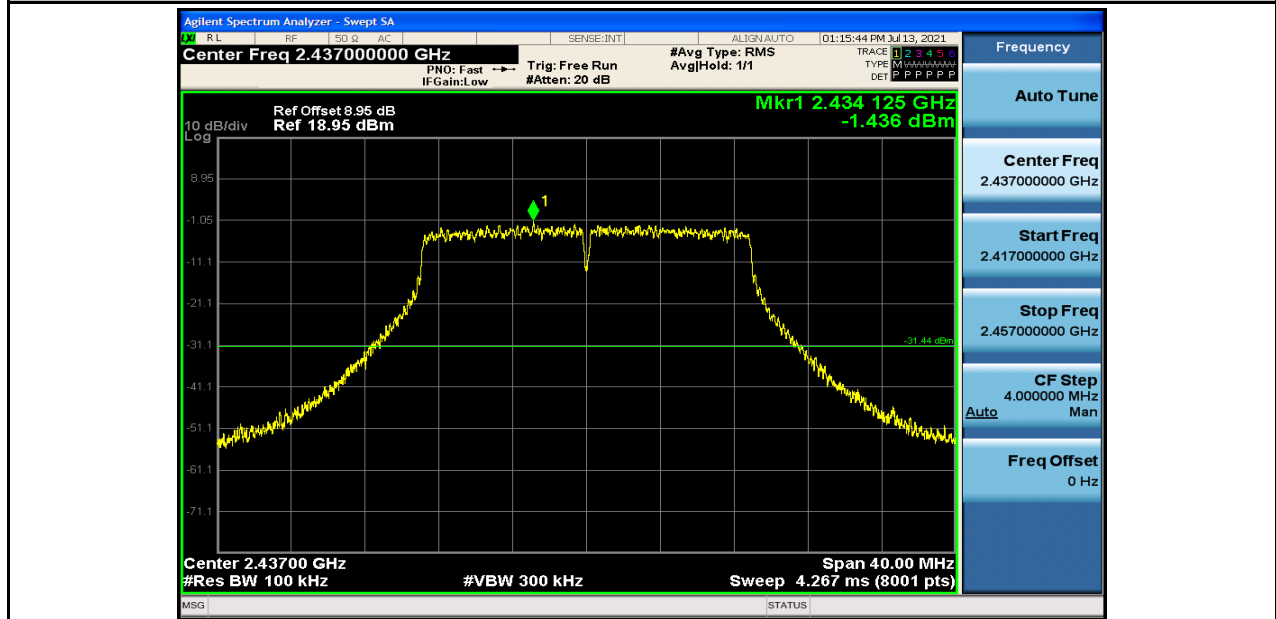
RF Conducted Spurious Emissions_11N20SISO_2437
