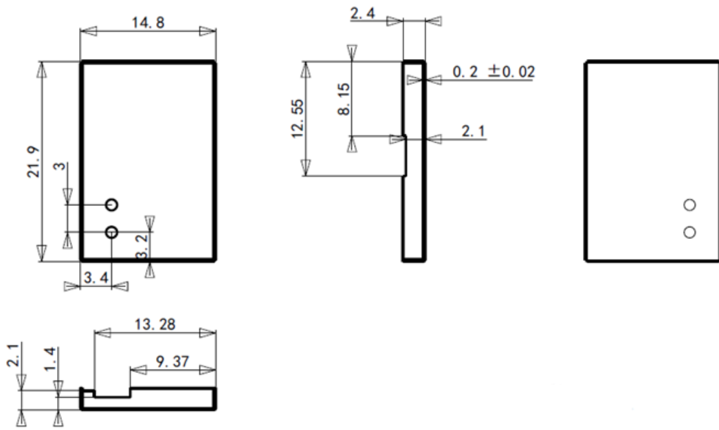
Fig 6 BL3372-P Dimensions of shielding case
