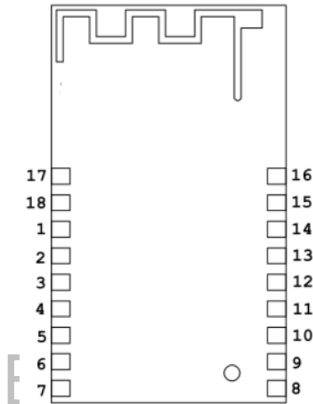
Fig 1 BL3372-P pin sequence
