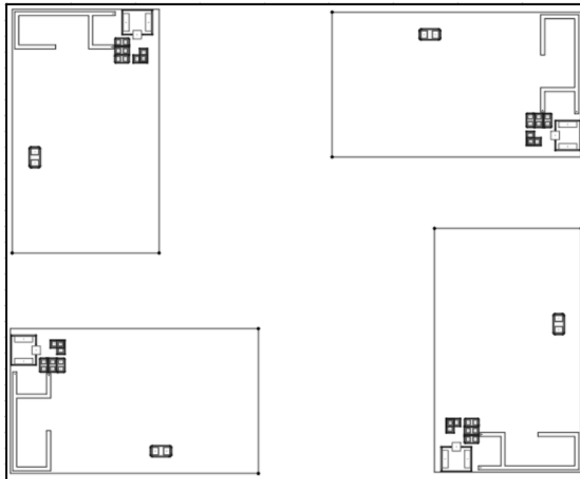
Fig 2 BL3372-P Recommended PCB layout
