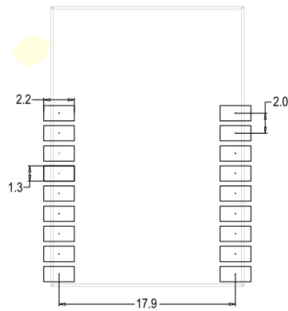
Fig 4 BL3372-P Recommended pad size
