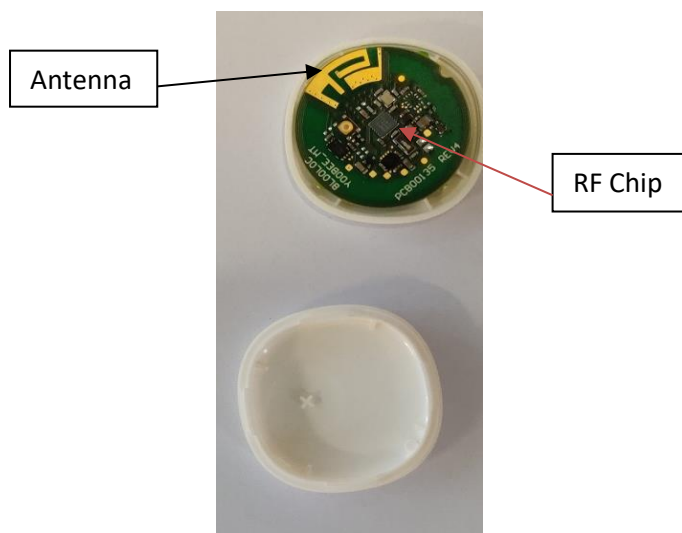
Figure 4: inside view PCB front
