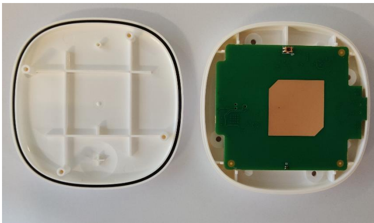
Figure 3: inside view PCB back
