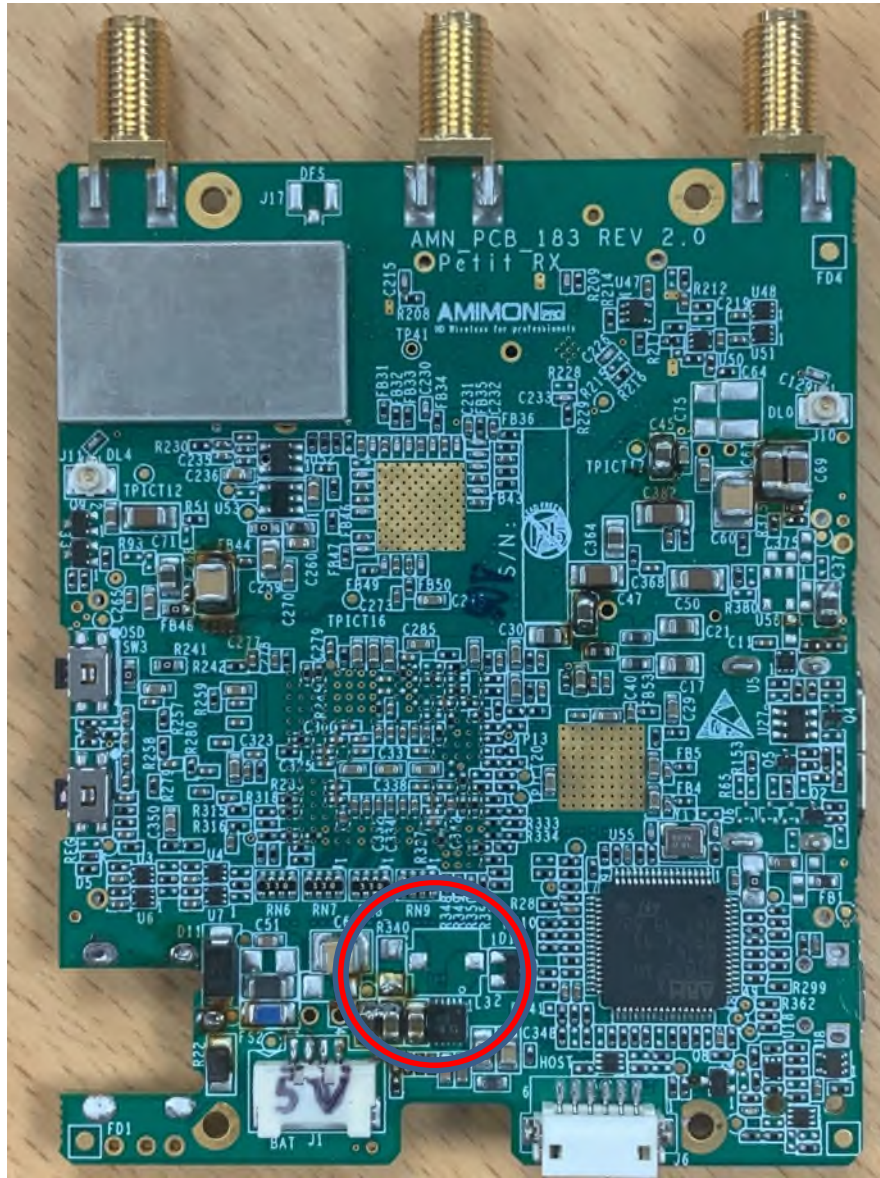
Figure 1 – EUT Internal Photo Back
