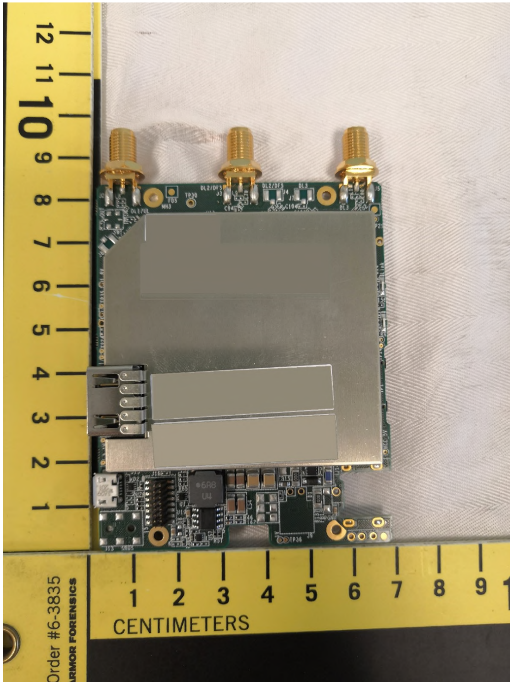
Figure 1 – EUT External Photo Front
