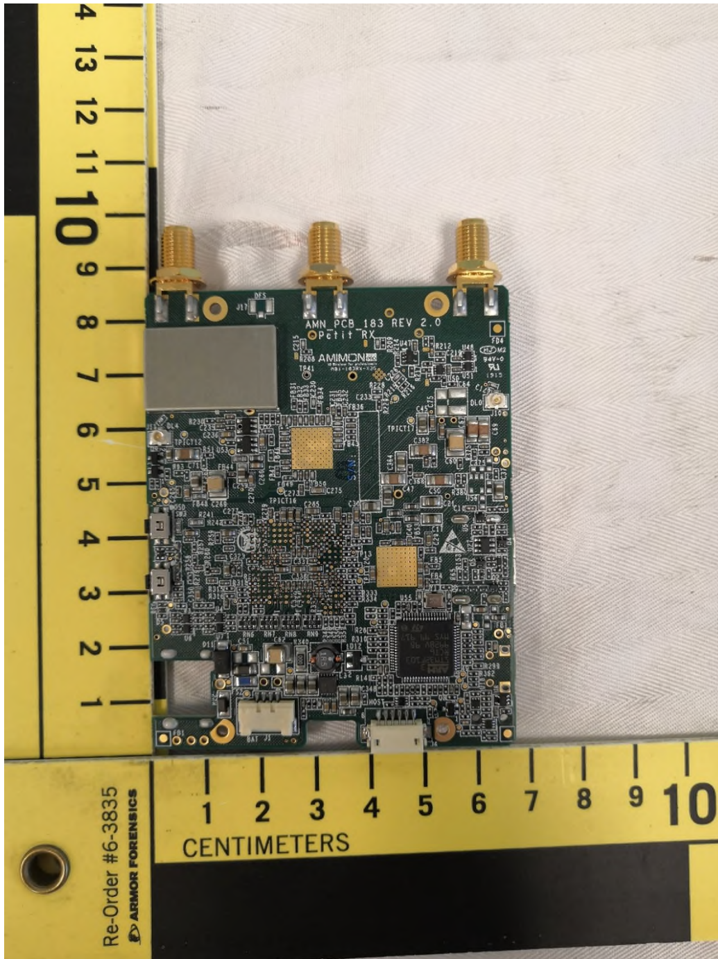
Figure 2 – EUT External Photo Back
