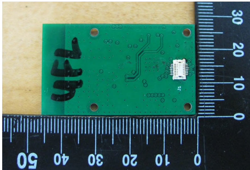
Figure 2 – EUT Internal Photo Back
