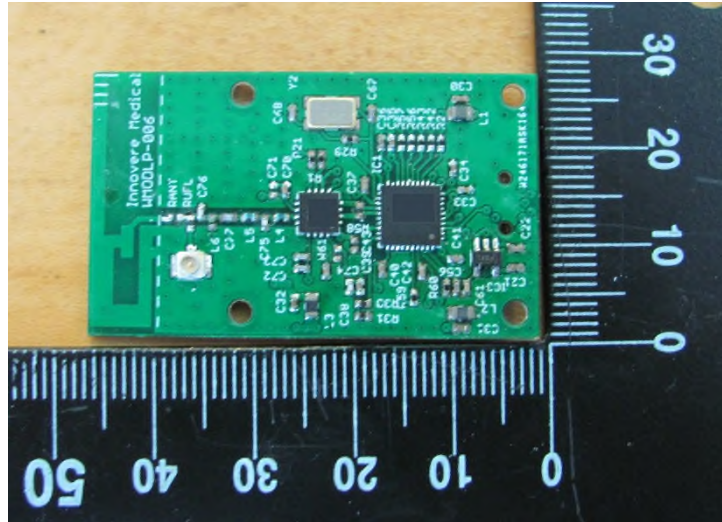
Figure 1 – EUT Internal Photo Front
