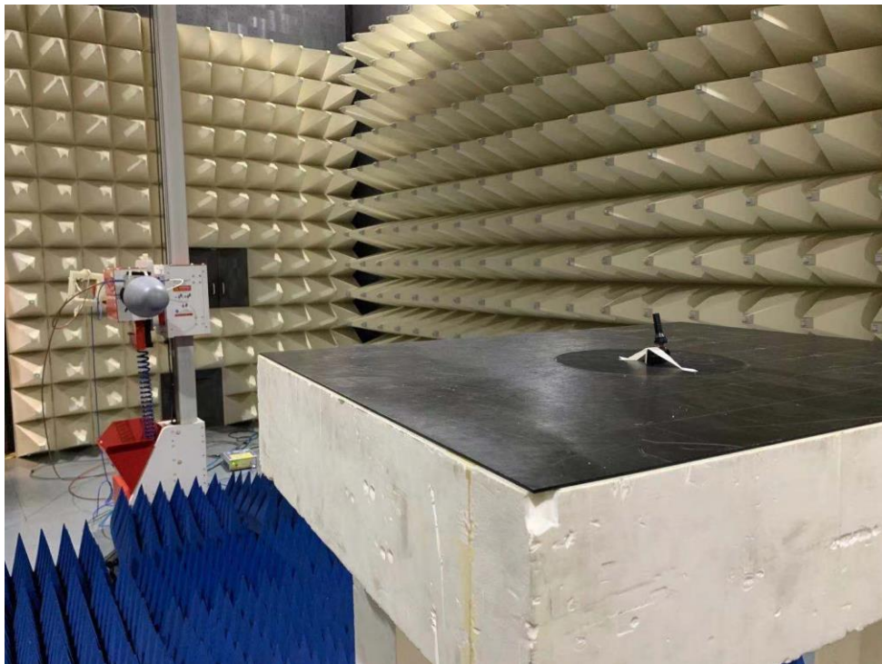
Photograph 2: Set-up photo for Radiated Emission, 1GHz - 4GHz
