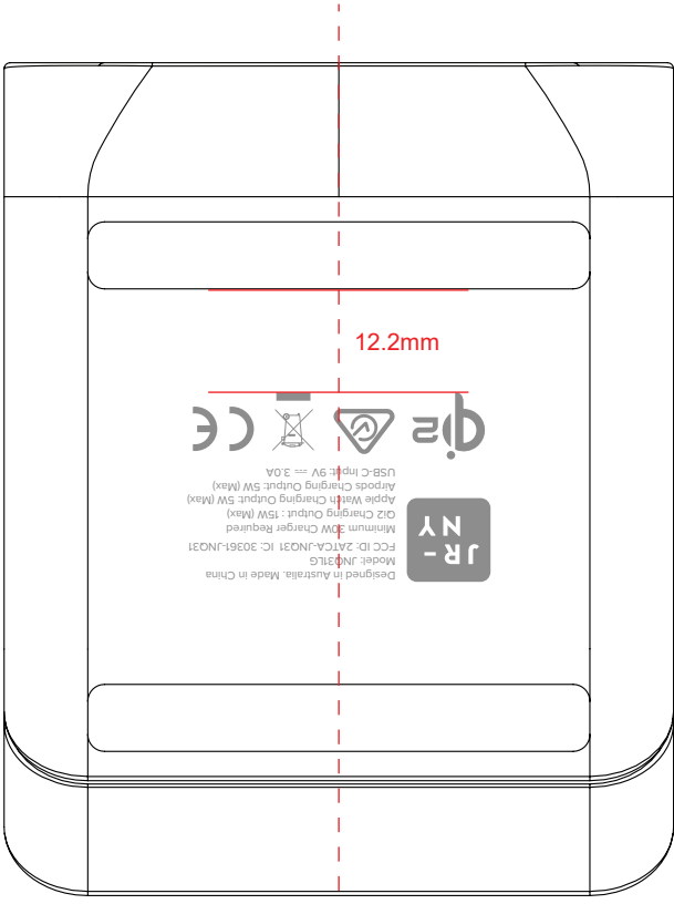
BASE VIEW
