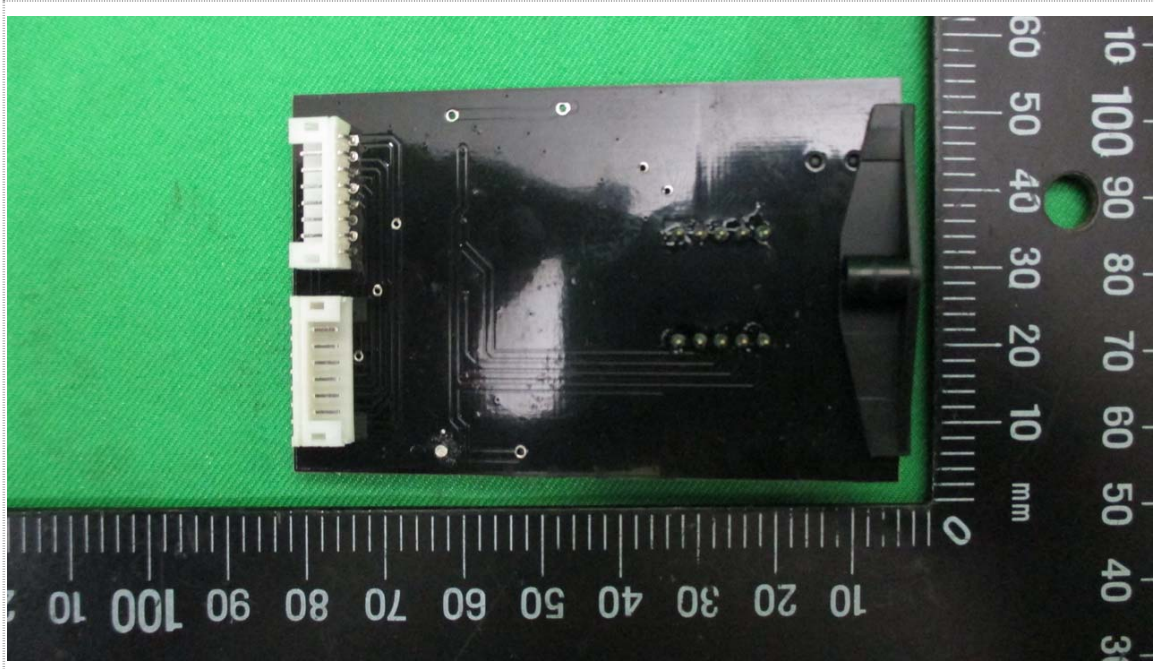
Rear View of Main Board
