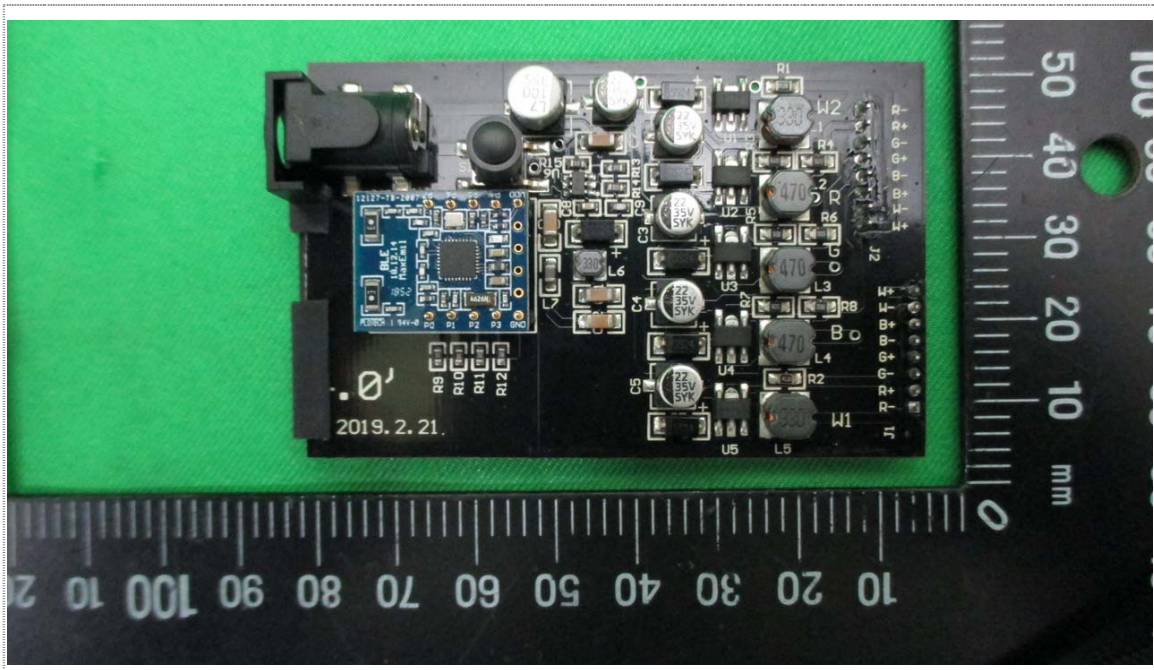
Front View of Main Board
