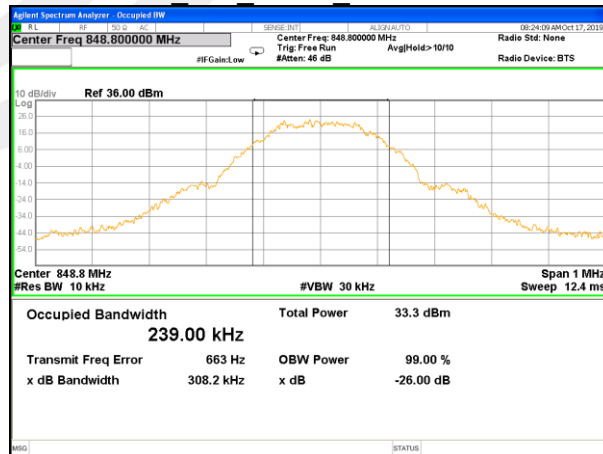
EGPRS 850 Higher 26BW and 99%
