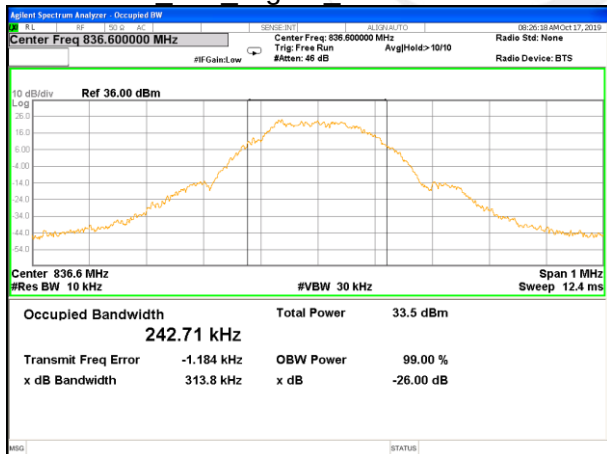
EGPRS 850 Middle 26BW and 99%
