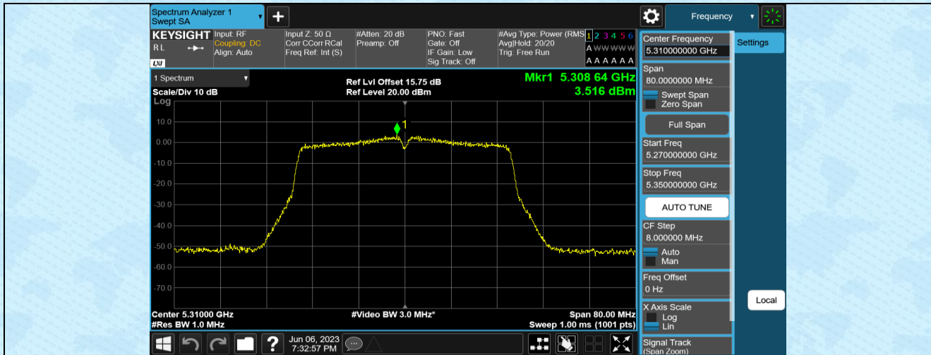
11AC40MIMO-Ant1-5310
