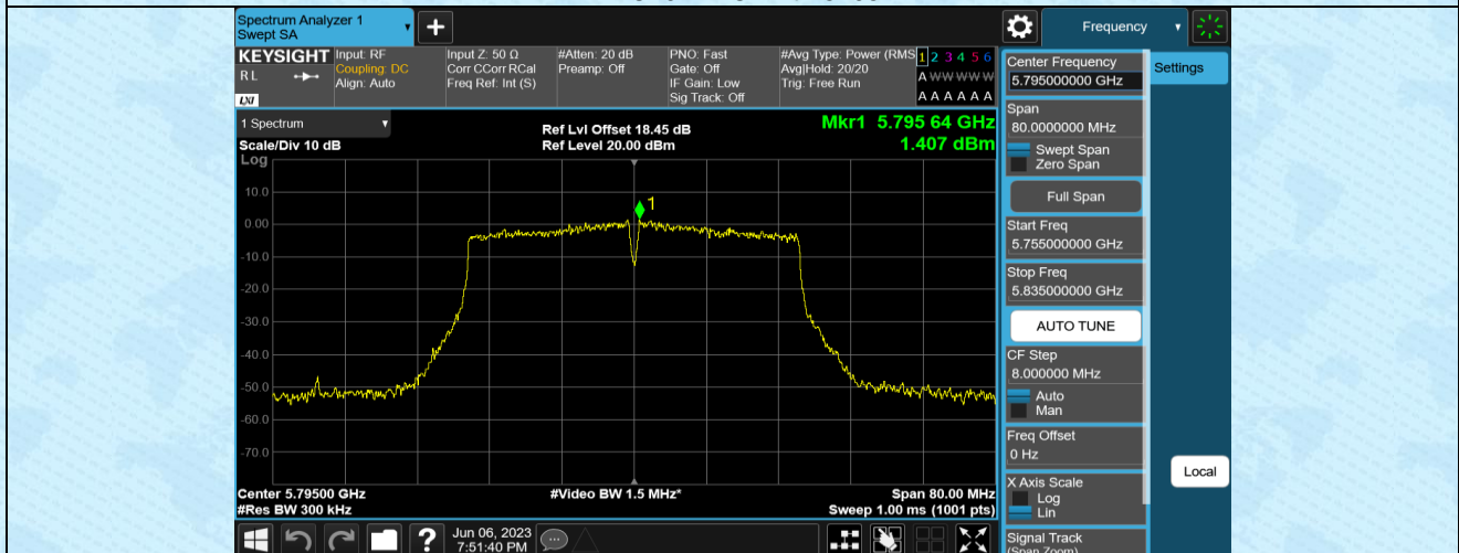
11AC40MIMO-Ant2-5795
