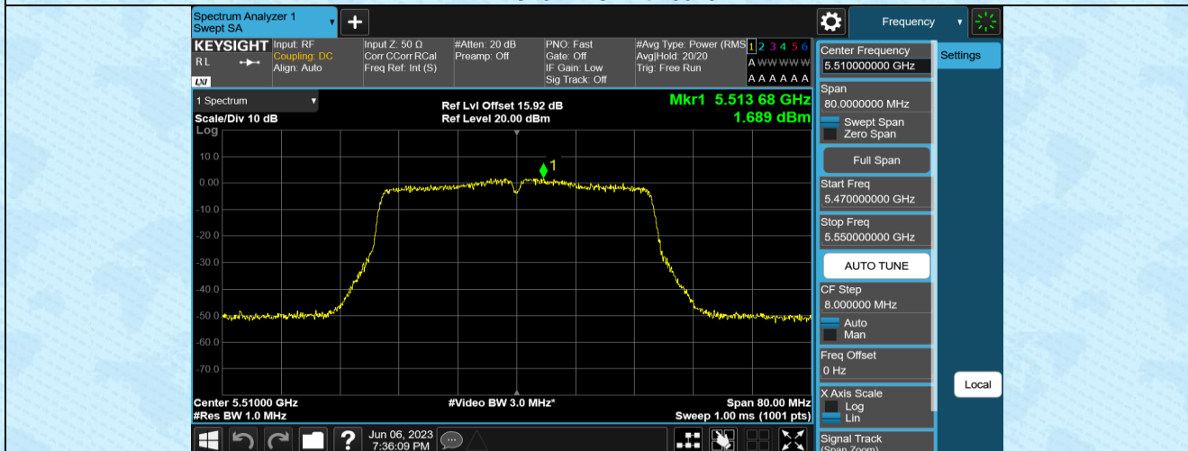
11AC40MIMO-Ant1-5510
