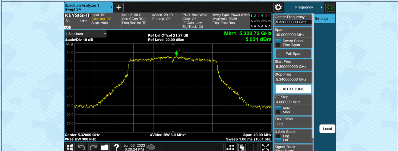
11AC20MIMO-Ant2-5320
