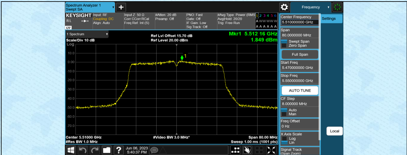
11N40MIMO-Ant2-5510
