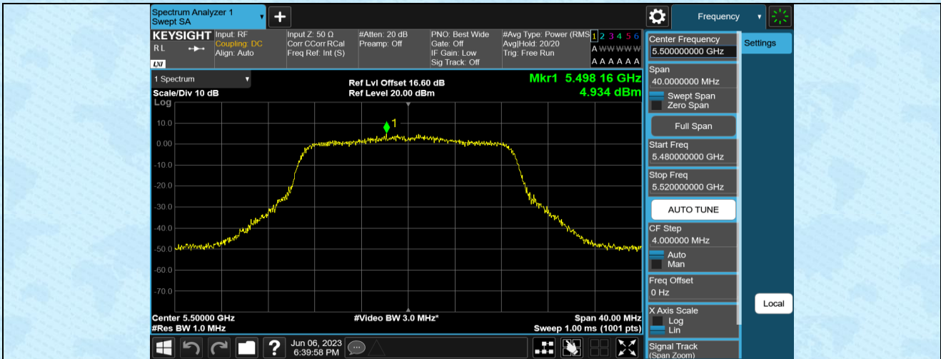
11AC20MIMO-Ant1-5500
