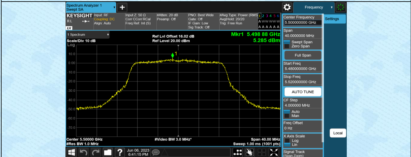
11AC20MIMO-Ant2-5500
