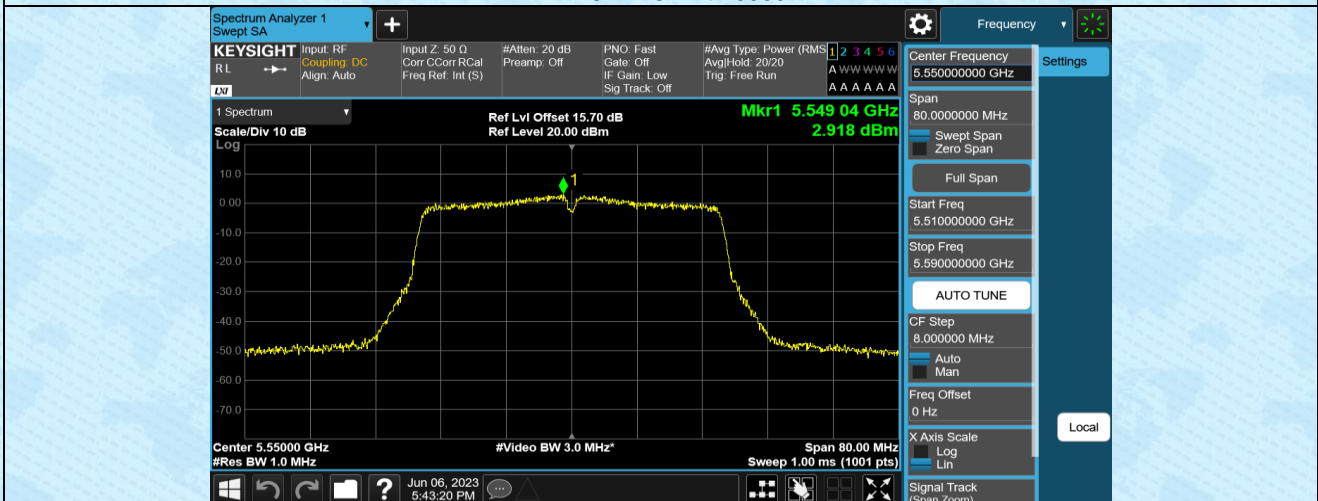
11N40MIMO-Ant2-5550
