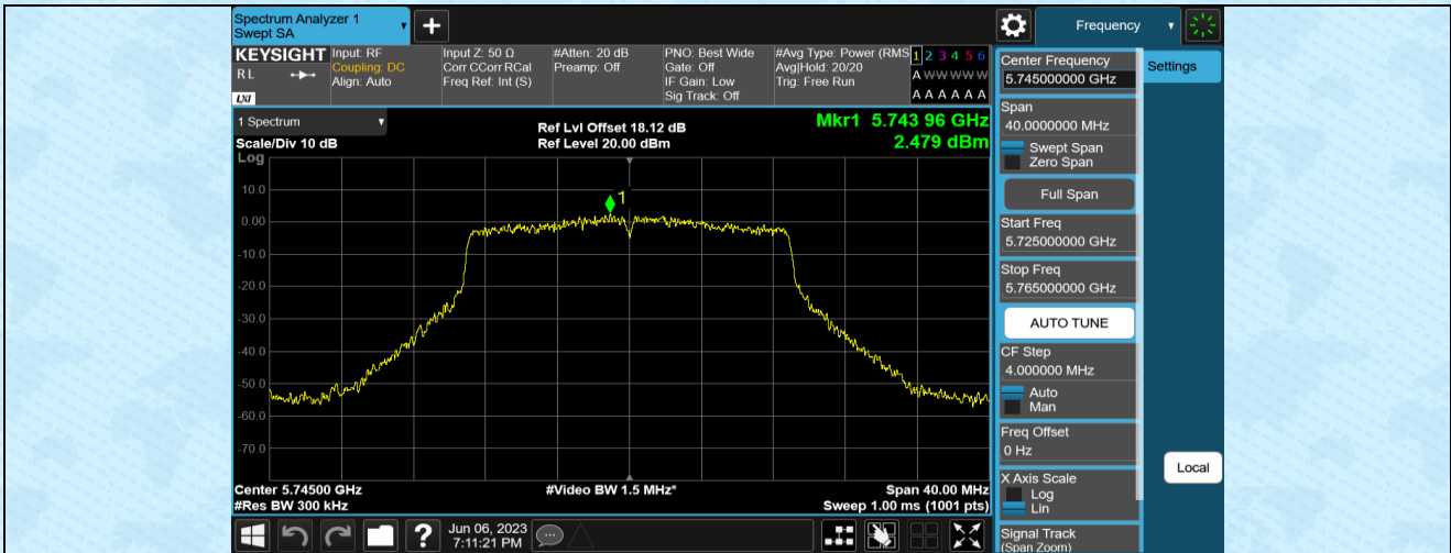
11AC20MIMO-Ant1-5745
