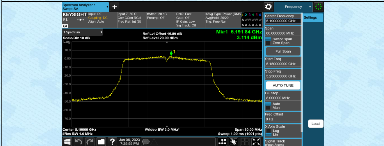
11AC40MIMO-Ant2-5190
