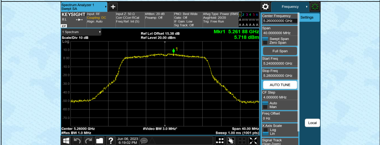
11AC20MIMO-Ant2-5260
