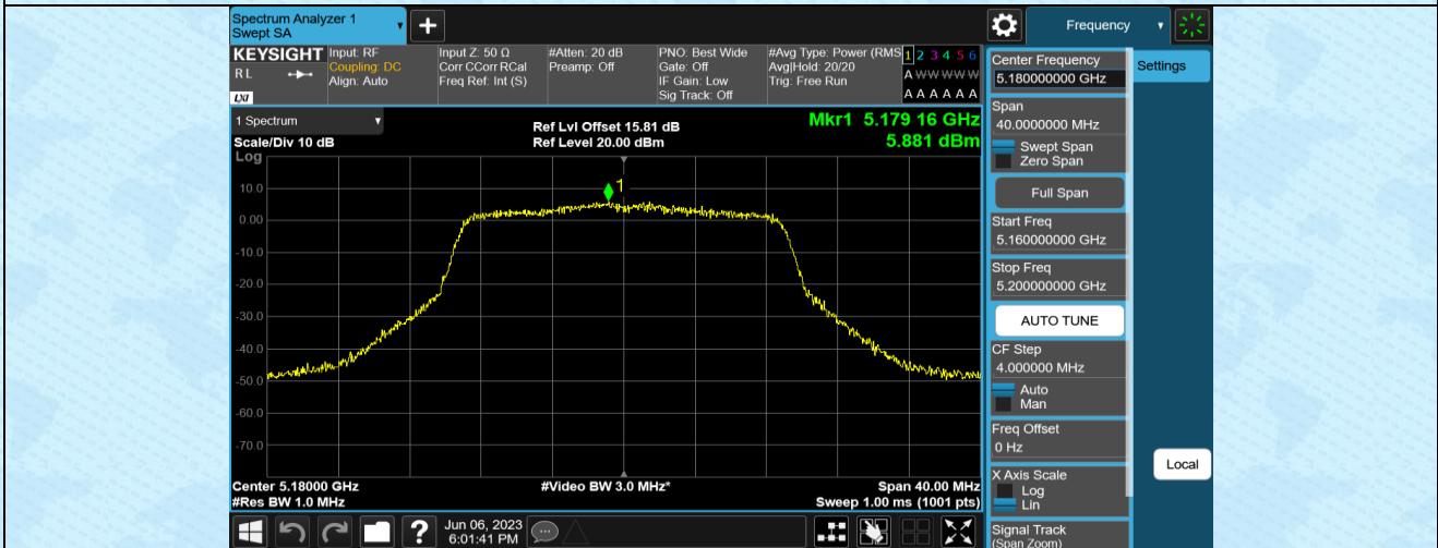
11AC20MIMO-Ant2-5180
