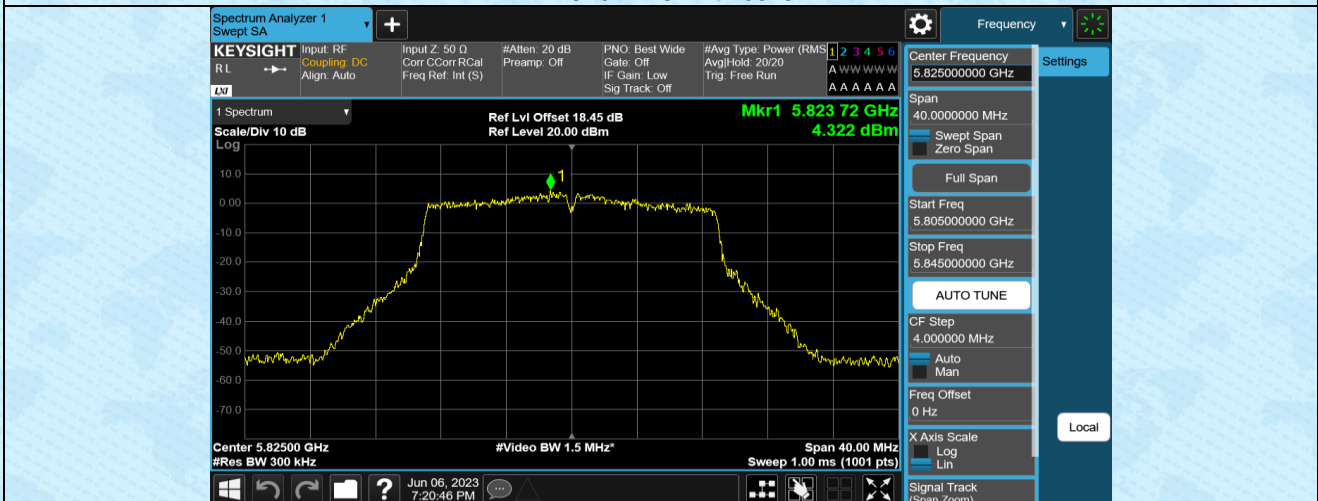
11AC20MIMO-Ant2-5825
