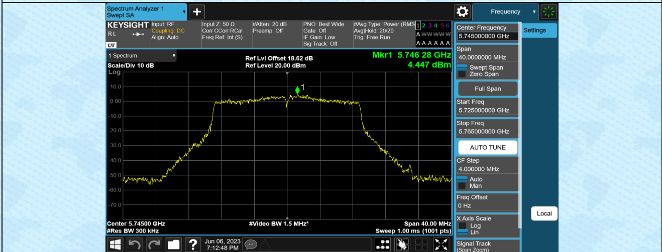
11AC20MIMO-Ant2-5745
