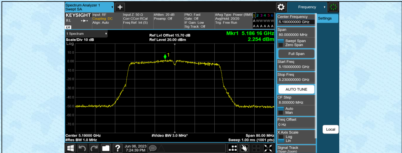
11AC40MIMO-Ant1-5190
