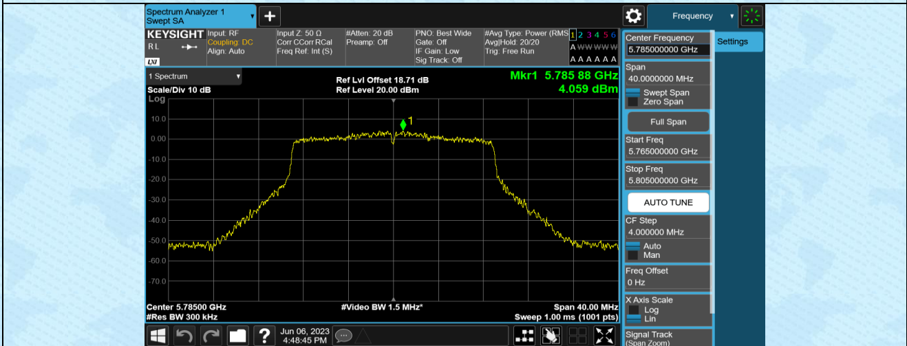
11N20MIMO-Ant1-5785
