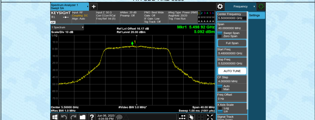
11A-CDD-Ant1-5500
