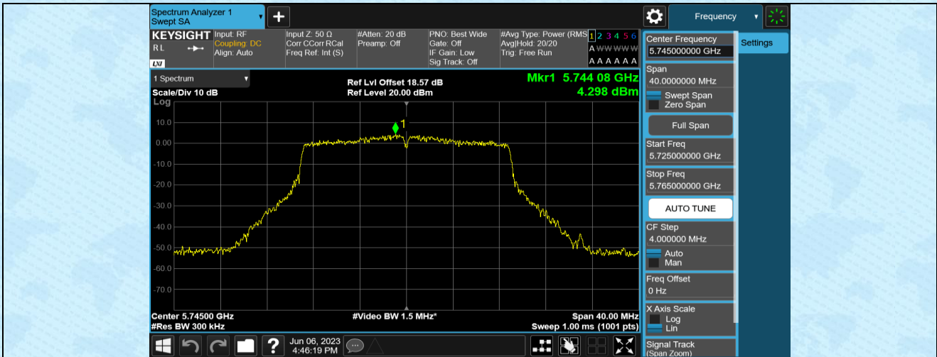
11N20MIMO-Ant2-5745
