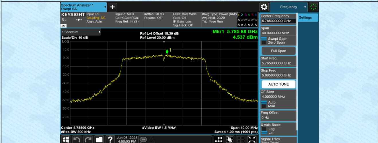
11N20MIMO-Ant2-5785
