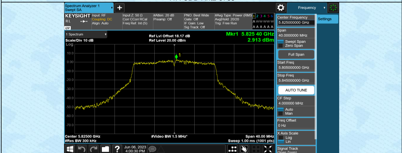
11A-CDD-Ant1-5825
