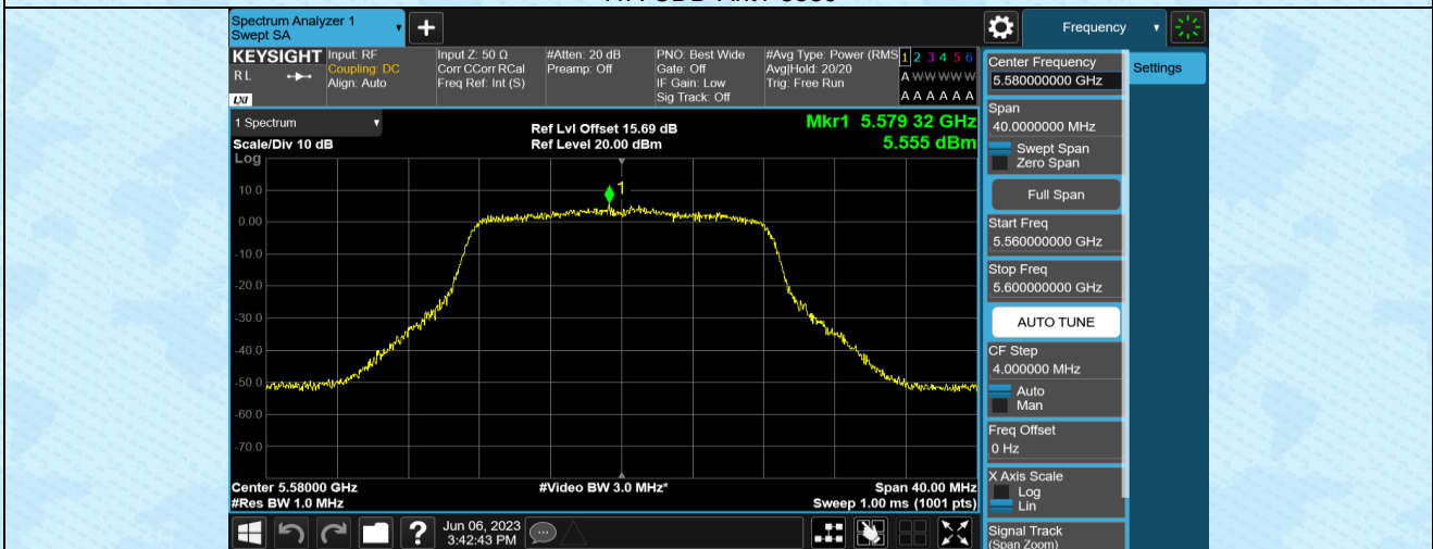
11A-CDD-Ant2-5580
