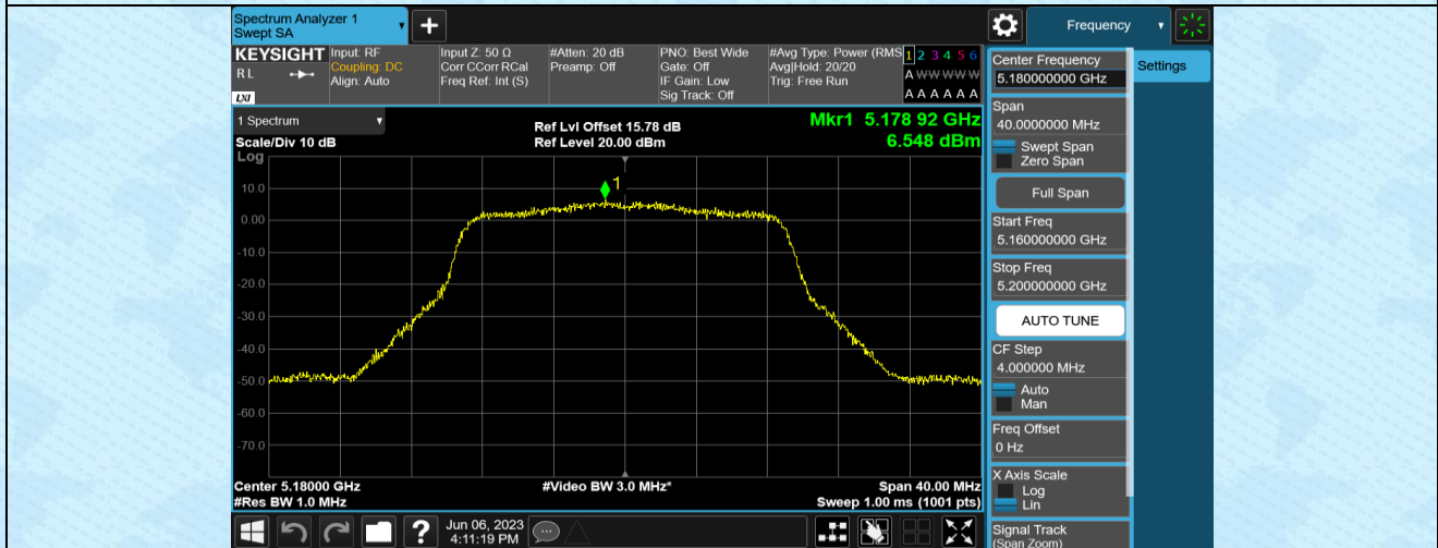
11N20MIMO-Ant2-5180
