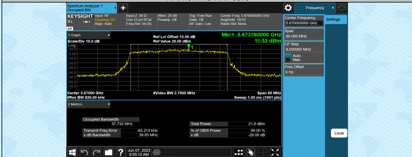
11AX40MIMO-Ant2-5670
