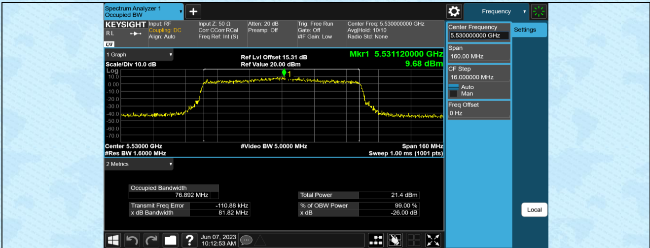
11AX80MIMO-Ant2-5530
