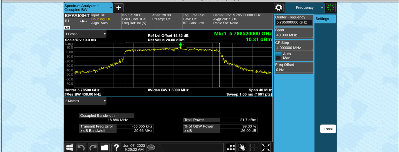
11AX20MIMO-Ant2-5785
