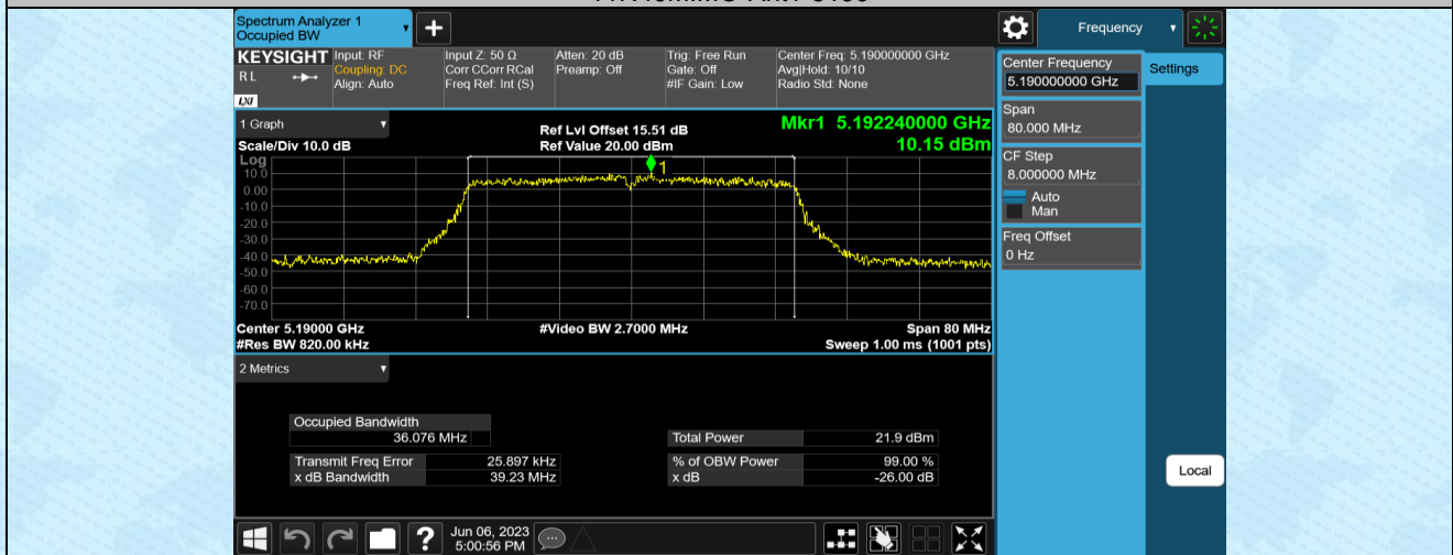
11N40MIMO-Ant2-5190
