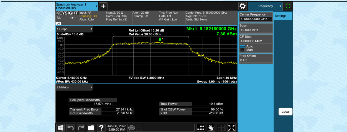
11AC20MIMO-Ant1-5180
