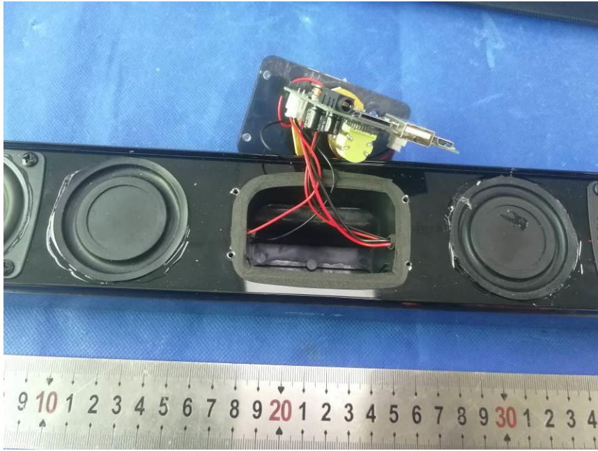
PCB ANTENNA
