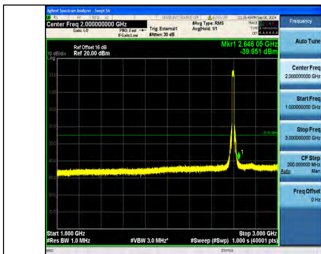
Band38_20MHz_QPSK_38000_100RB#0_18000~27000_18000~27000
