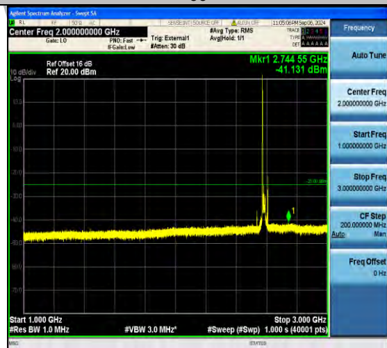
Band38_20MHz_16QAM_37850_1RB#0_18000~27000_18000~27000
