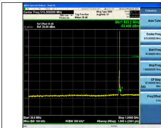
Band5_3MHz_16QAM_20415_1RB#14_3000~10000_3000~1000000
