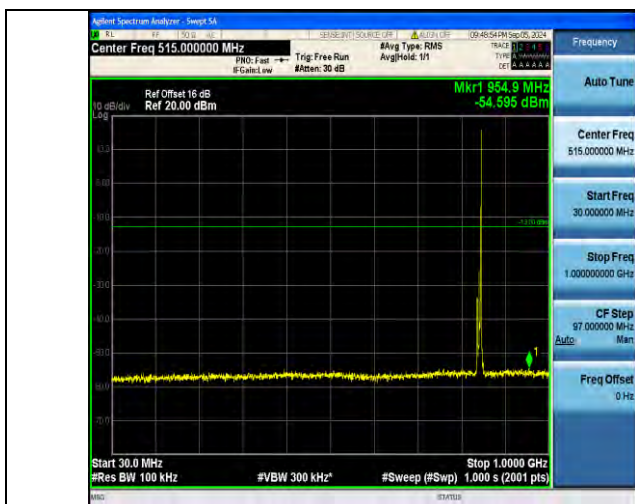
Band5_5MHz_64QAM_20625_1RB#24_3000~10000_3000~1000000
