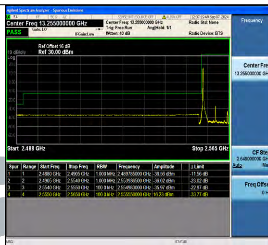
Band41 10MHz 64QAM 40290 50RB#0
