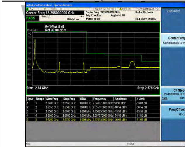
Band41_15MHz_QPSK_41165_75RB#0
