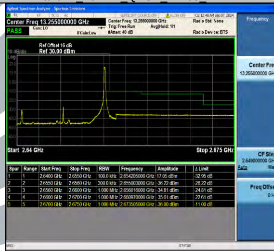
Band41_15MHz_64QAM_40315_1RB#0
