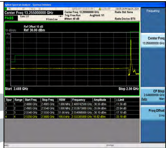
Band41 5MHz 64QAM 40265 25RB#0
