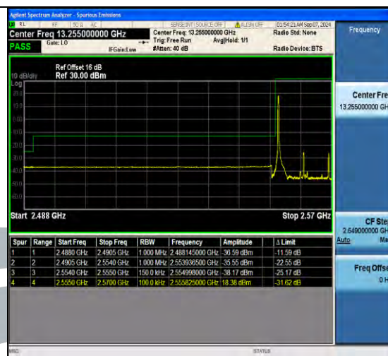
Band41_15MHz_QPSK_40315_75RB#0
