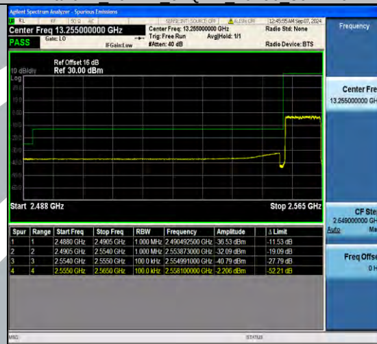
Band41 10MHz 64QAM 41190 1RB#49
