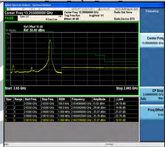
Band41 5MHz 64QAM 41215 25RB#0
