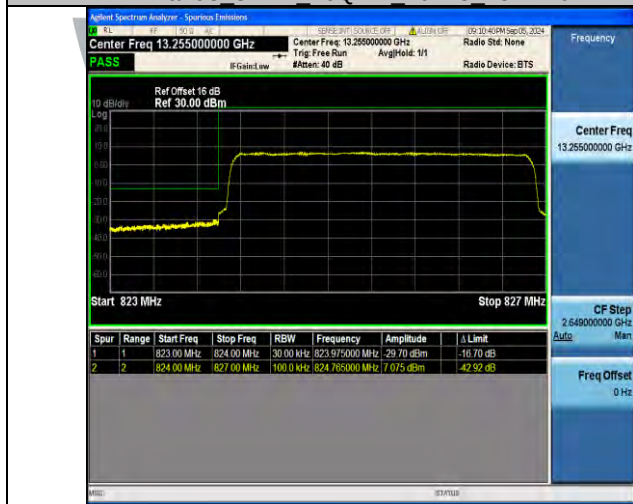
Band5 3MHz 16QAM 20635 1RB#14
