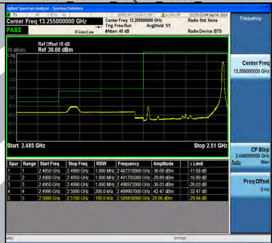
Band7 10MHz 16QAM 20800 50RB#49
