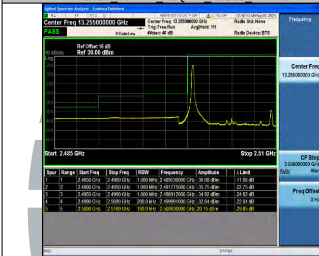
Band7 10MHz 16QAM 20800 50RB#0
