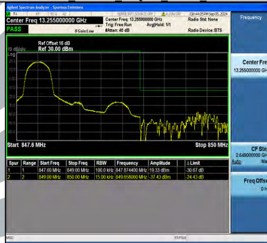
Band5 1.4MHz 64QAM 20643 1RB#5
