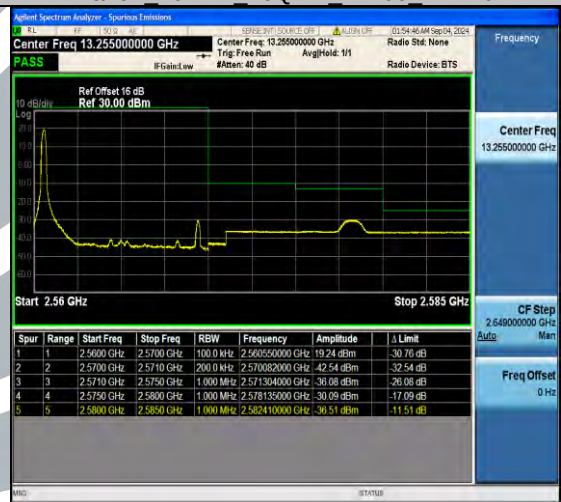
Band7 10MHz 16QAM 21400 50RB#0
