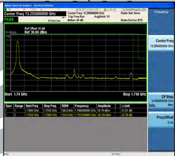
Band4 15MHz 64QAM 20325 75RB#0
