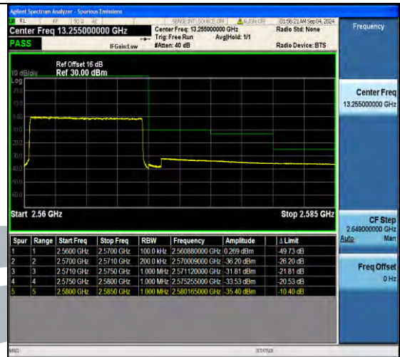
Band7 10MHz 16QAM 20800 1RB#49
