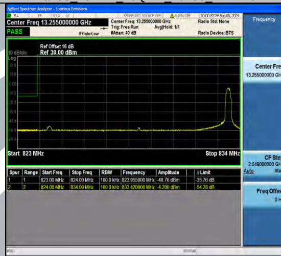
Band5 10MHz 16QAM 20450 1RB#49
