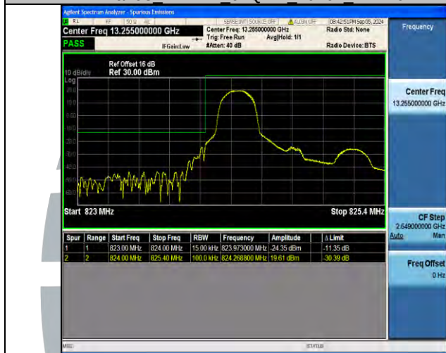
Band5 1.4MHz 64QAM 20407 6RB#0
