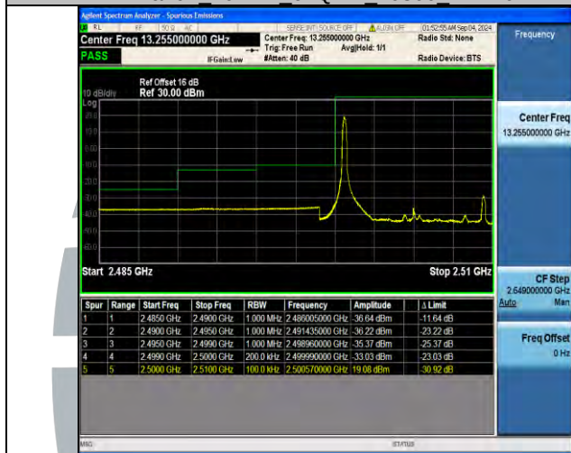
Band7 10MHz 64QAM 20800 50RB#0
