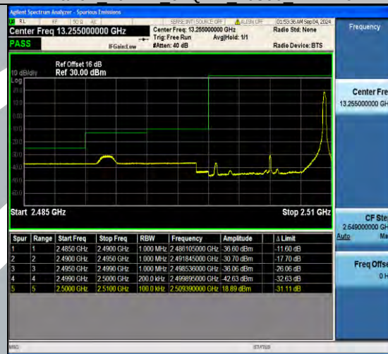
Band7 10MHz 64QAM 20800 1RB#49
