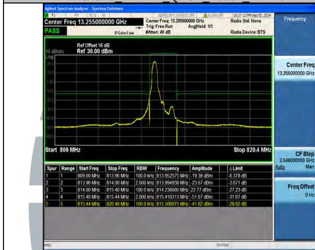
Band26 1.4MHz QPSK 26697 6RB#0
