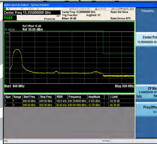
Band5 3MHz 16QAM 20635 15RB#0
