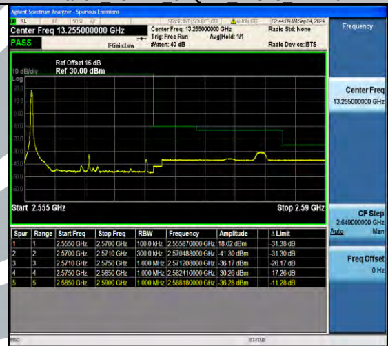
Band7 15MHz 64QAM 21375 75RB#0
