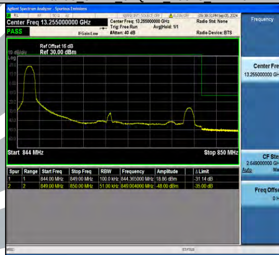
Band5 5MHz 64QAM 20625 25RB#0
