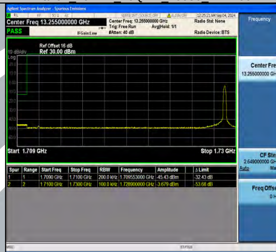
Band4 20MHz 16QAM 20050 100RB#99
