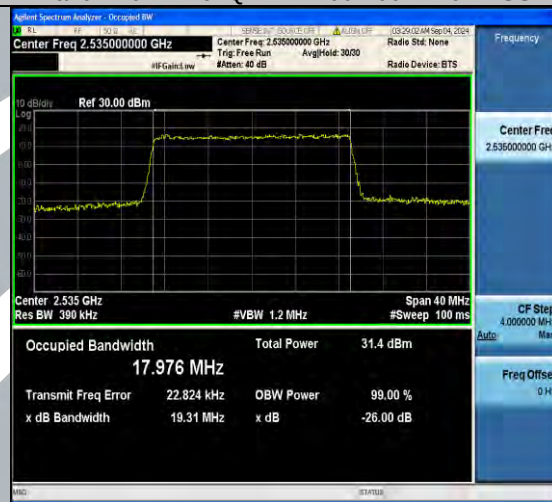
Band7-20MHz-16QAM-20850-100RB#0-PASS
