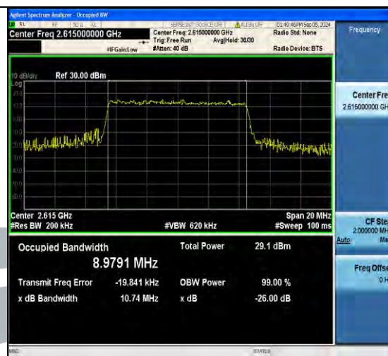
Band38-10MHz-16QAM-38000-50RB#0-PASS
