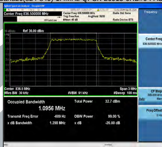
Band26(824-849)-1.4MHz-QPSK-26915-6RB#0-PASS
