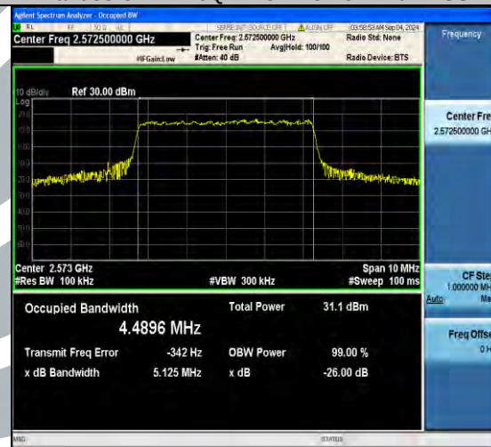
Band38-5MHz-16QAM-38225-25RB#0-PASS
