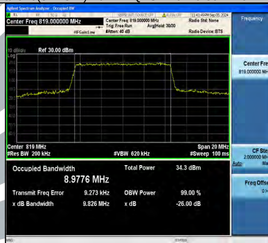
Band26(814-824)-10MHz-16QAM-26740-50RB#0-PASS
