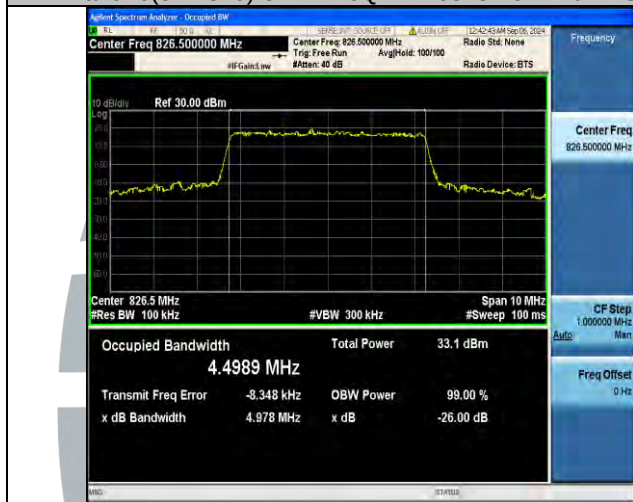
Band26(824-849)-5MHz-16QAM-27015-25RB#0-PASS
