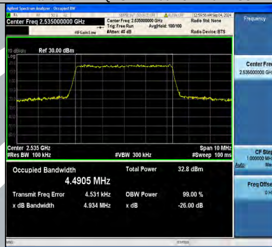
Band7-5MHz-QPSK-21100-25RB#0-PASS
