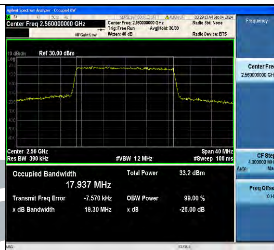
Band7-20MHz-64QAM-21100-100RB#0-PASS
