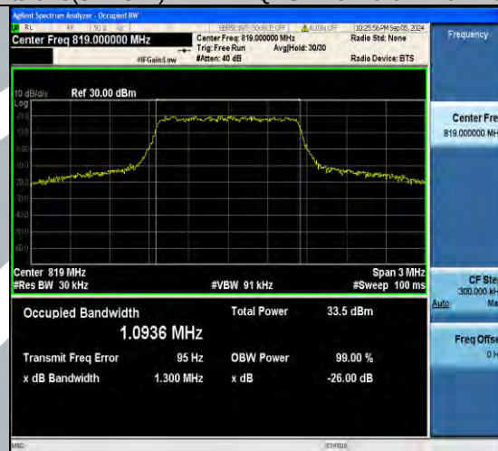
Band26(814-824)-1.4MHz-QPSK-26740-6RB#0-PASS
