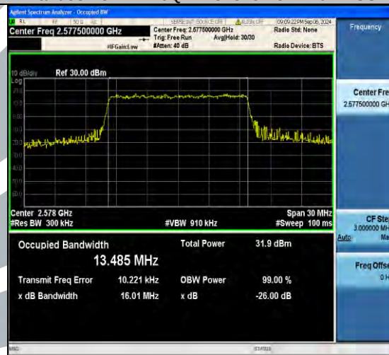
Band38-15MHz-16QAM-38175-75RB#0-PASS
