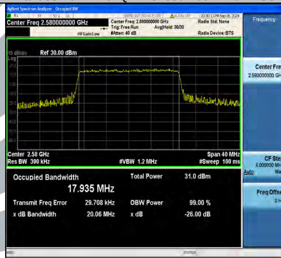
Band38-20MHz-64QAM-38150-100RB#0-PASS
