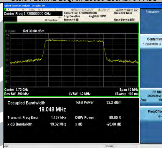
Band4-20MHz-16QAM-20300-100RB#0-PASS
