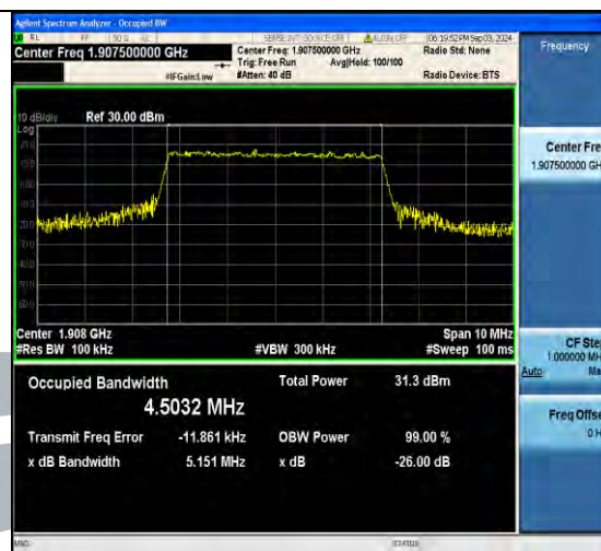
Band2-5MHz-16QAM-18900-25RB#0-PASS
