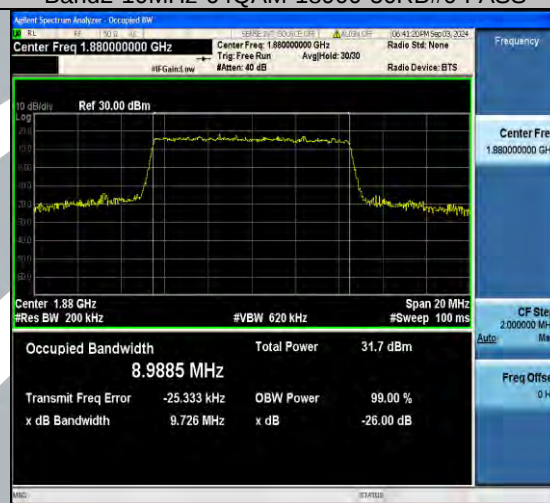
Band2-10MHz-16QAM-18650-50RB#0-PASS
