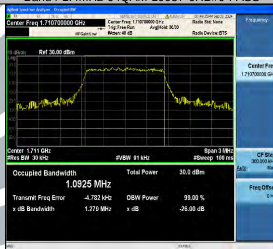
Band4-1.4MHz-64QAM-20393-6RB#0-PASS
