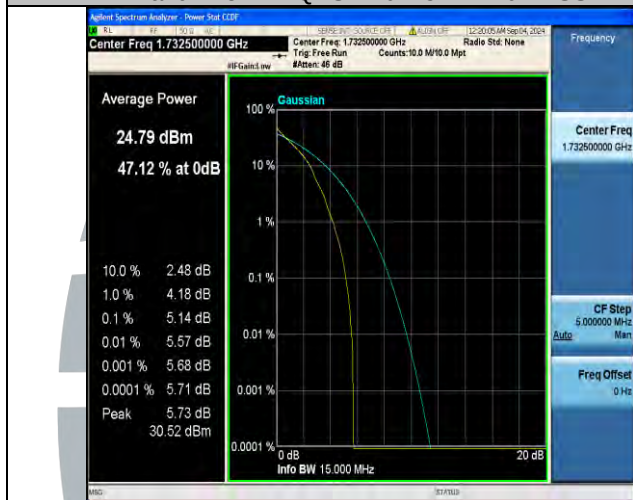
Band4-15MHz-QPSK-17325-1RB#0-PASS
