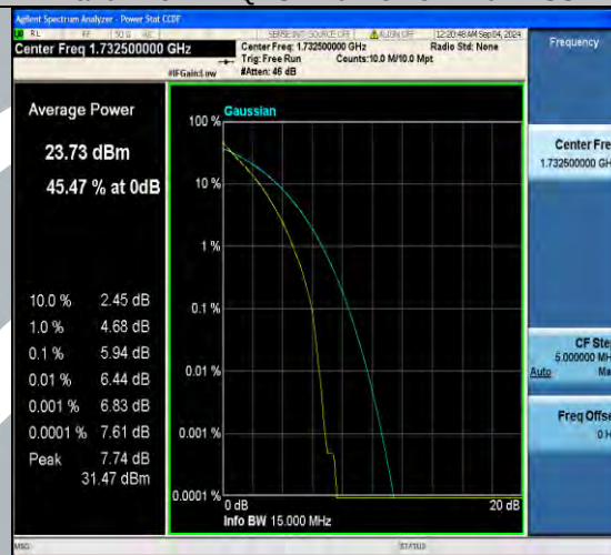
Band4-15MHz-QPSK-17325-75RB#0-PASS
