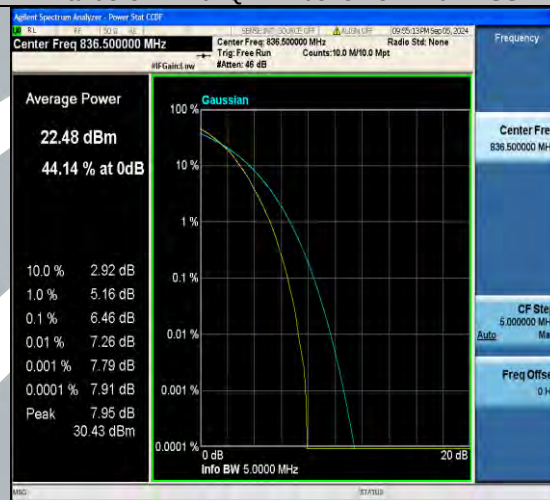
Band5-5MHz-64QAM-20625-25RB#0-PASS
