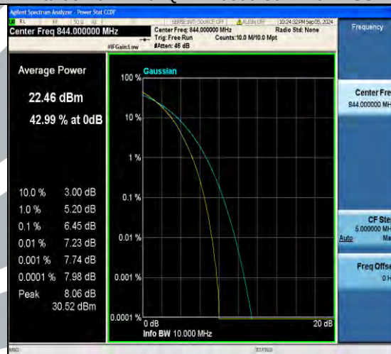
Band5-10MHz-16QAM-20450-50RB#0-PASS
