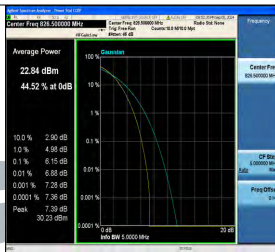
Band5-5MHz-64QAM-20525-25RB#0-PASS
