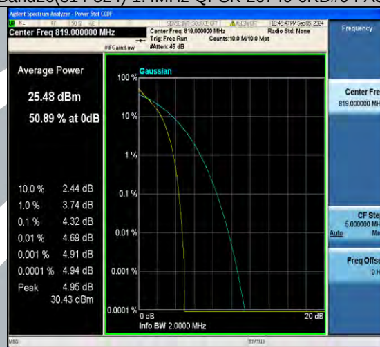
Band26(814-824)-1.4MHz-QPSK-26783-6RB#0-PASS
