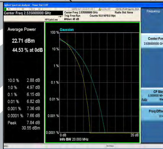
Band7-20MHz-16QAM-21350-100RB#0-PASS
