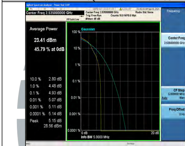
Band7-5MHz-16QAM-21425-1RB#0-PASS
