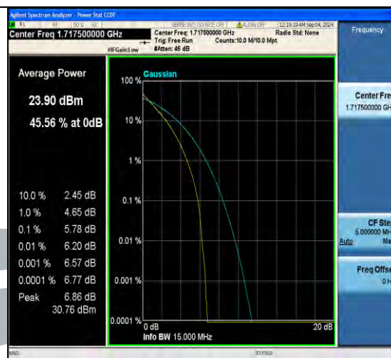
Band4-15MHz-QPSK-20175-75RB#0-PASS
