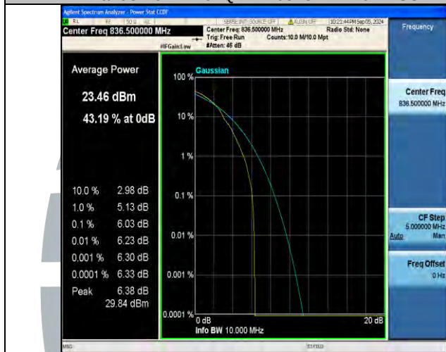
Band5-10MHz-64QAM-20600-1RB#0-PASS
