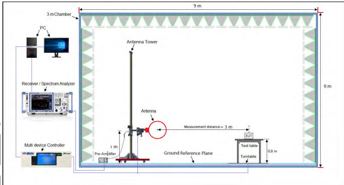
Figure 1. Below 30MHz
