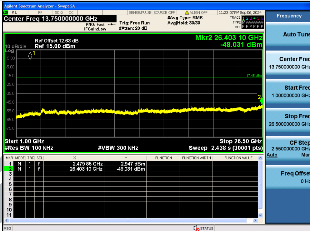
BLE_125K-Ant1-2480-1000~26500-PASS
