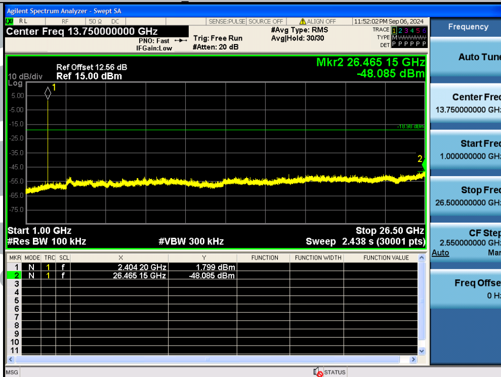
BLE_2M-Ant1-2404-1000~26500-PASS
