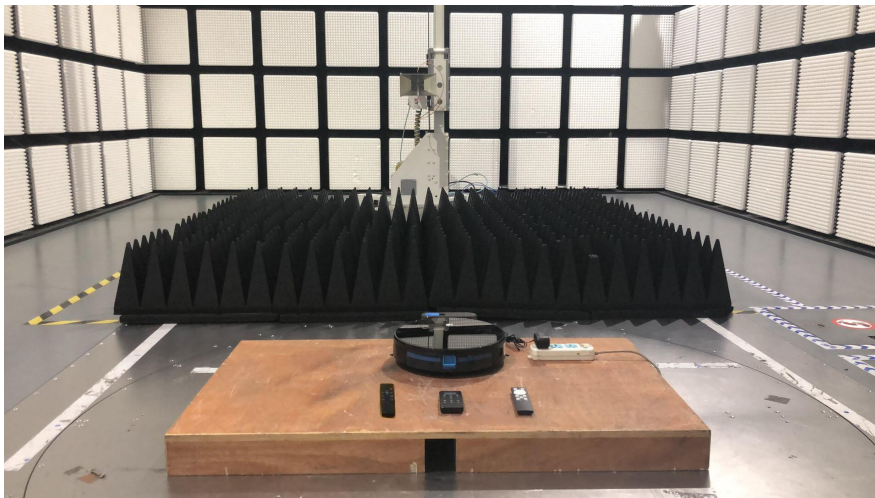
Radiated Emissions (Above 1G)
