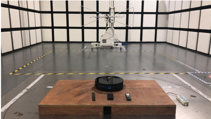
Radiated Emissions (30MHz~1000MHz)
