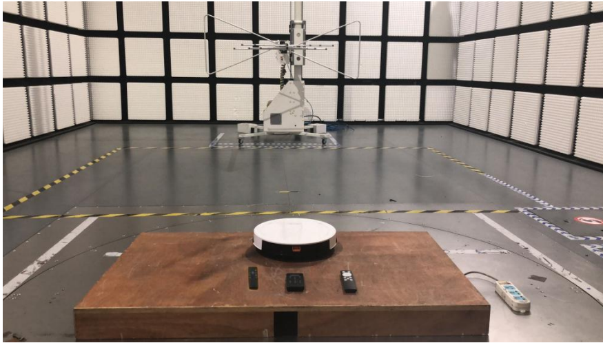
Radiated Emissions (30MHz~1000MHz)
