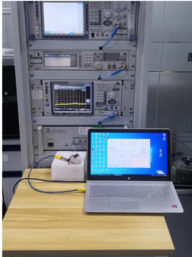
Conducted Emission
