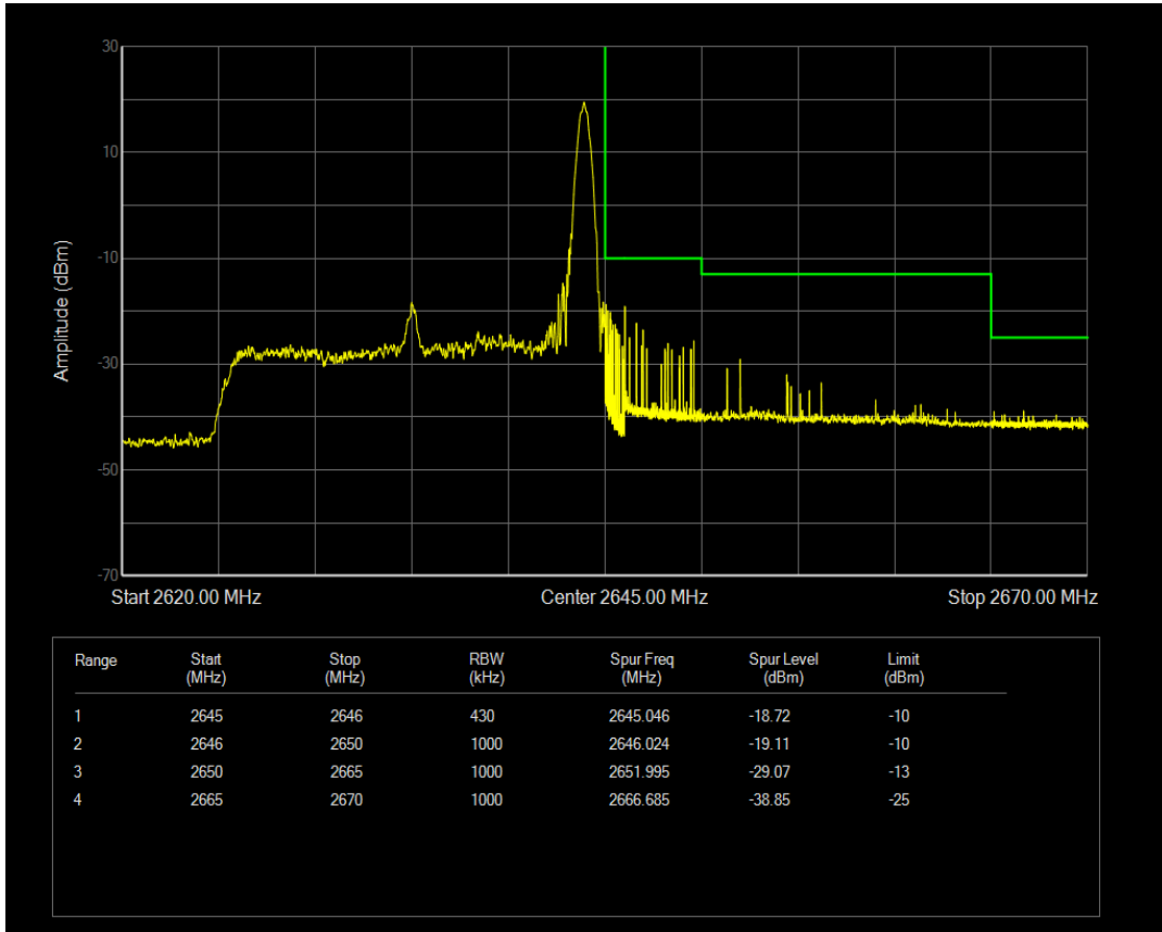
Band41 16QAM BW=20MHz Channel=41040 RB Size=100 Position=#0
