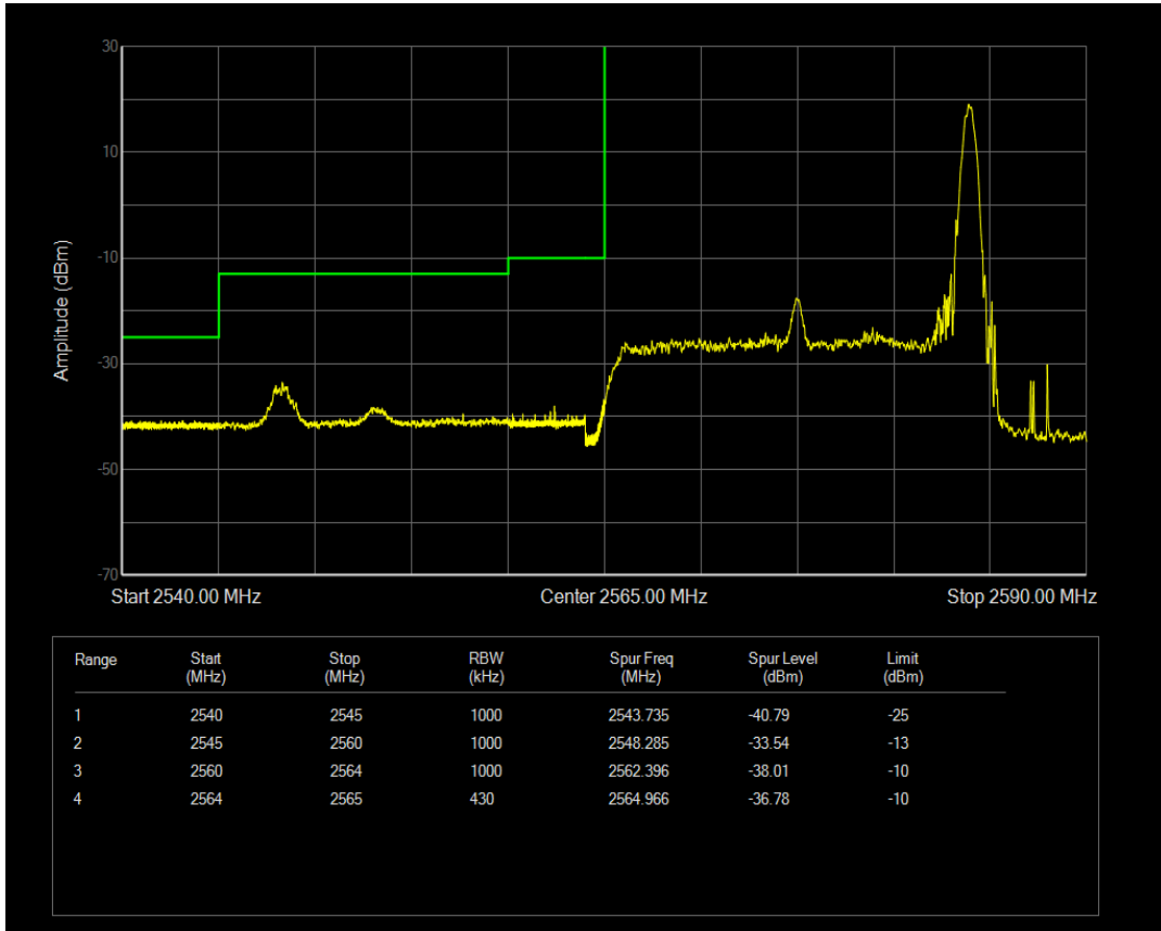
Band41 16QAM BW=20MHz Channel=40440 RB Size=100 Position=#0
