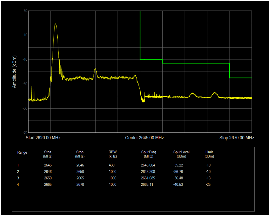
Band41 QPSK BW=20MHz Channel=41040 RB Size=1 Position=#Max
