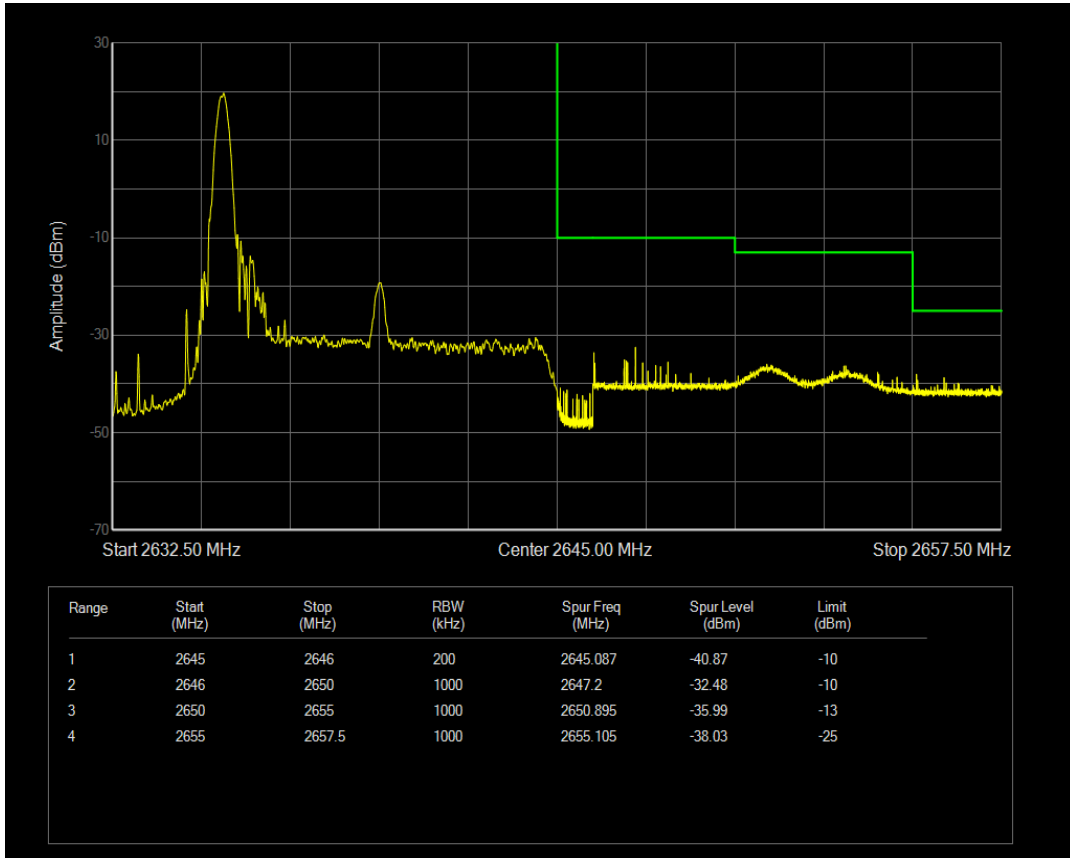
Band41 QPSK BW=10MHz Channel=41090 RB Size=1 Position=#Max
