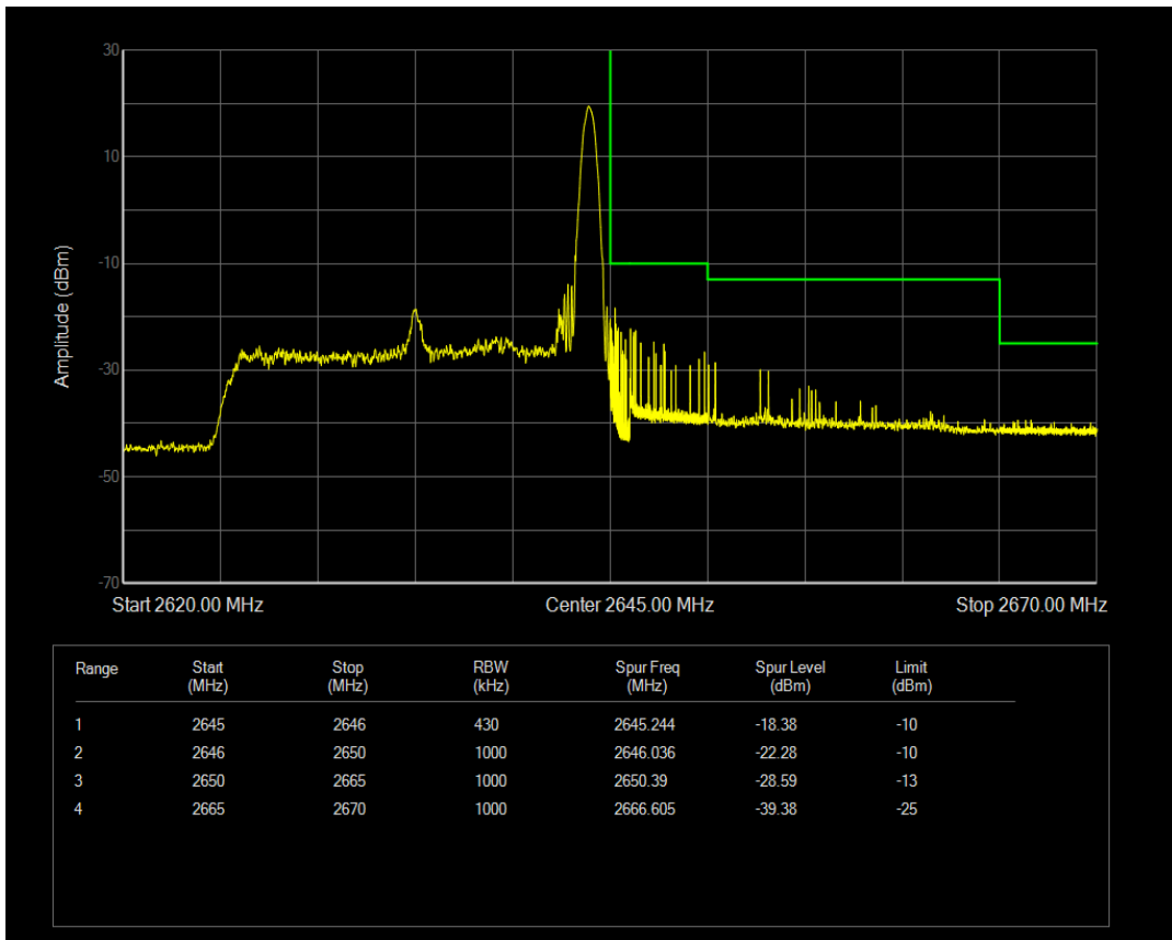
Band41 QPSK BW=20MHz Channel=41040 RB Size=100 Position=#0
