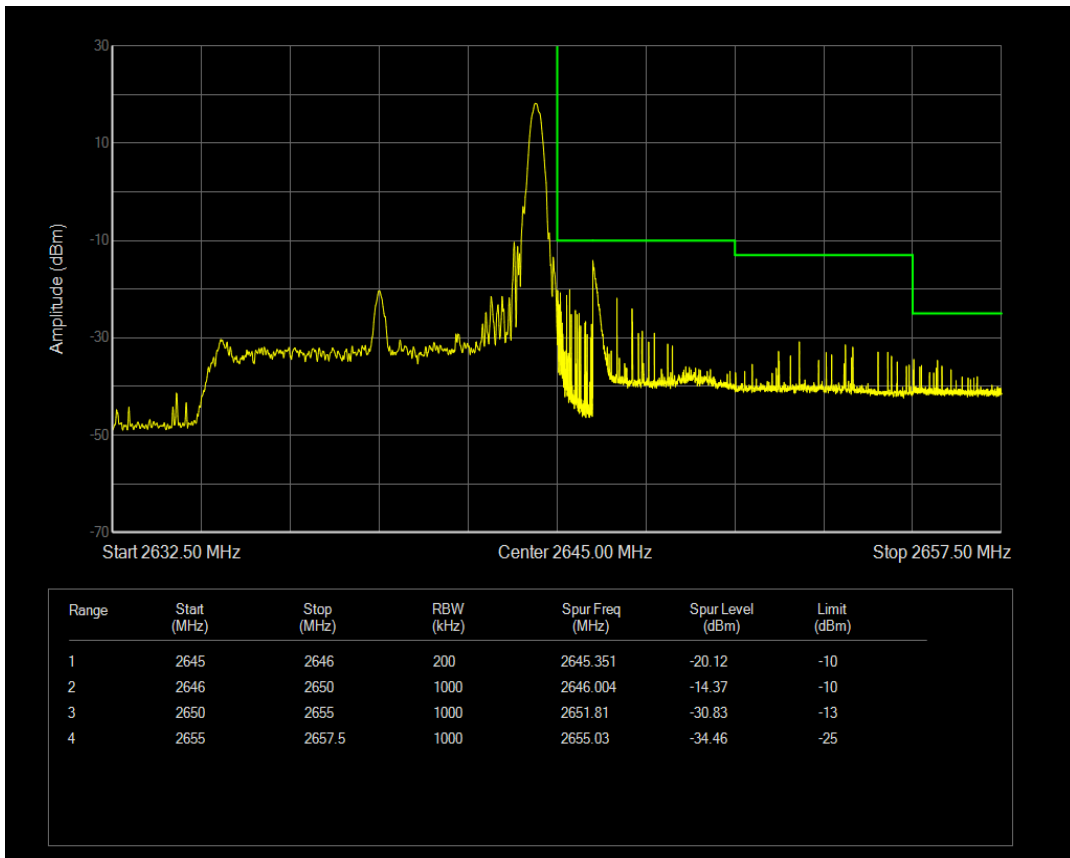
Band41 QPSK BW=10MHz Channel=41090 RB Size=50 Position=#0
