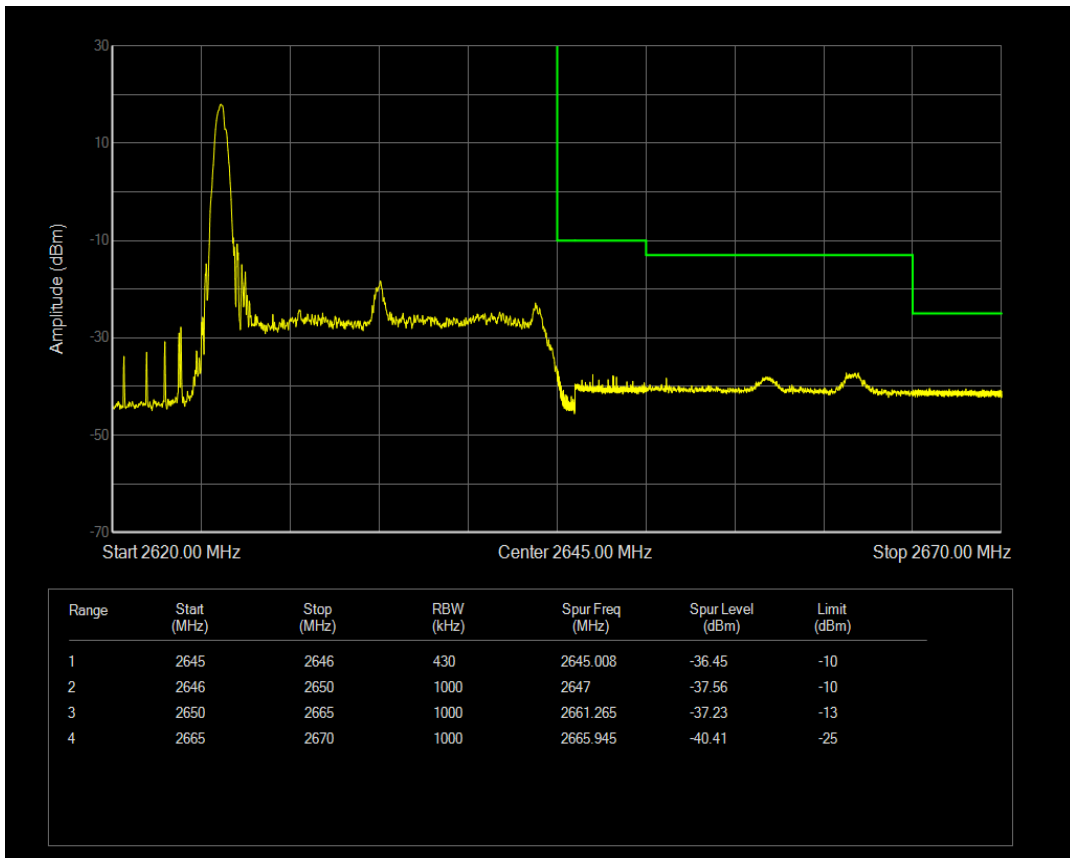
Band41 16QAM BW=20MHz Channel=41040 RB Size=1 Position=#Max
