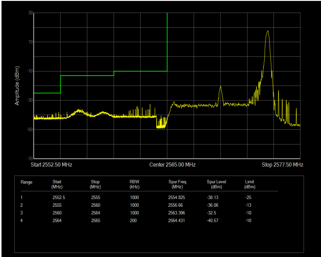
Band41 16QAM BW=10MHz Channel=40390 RB Size=50 Position=#0
