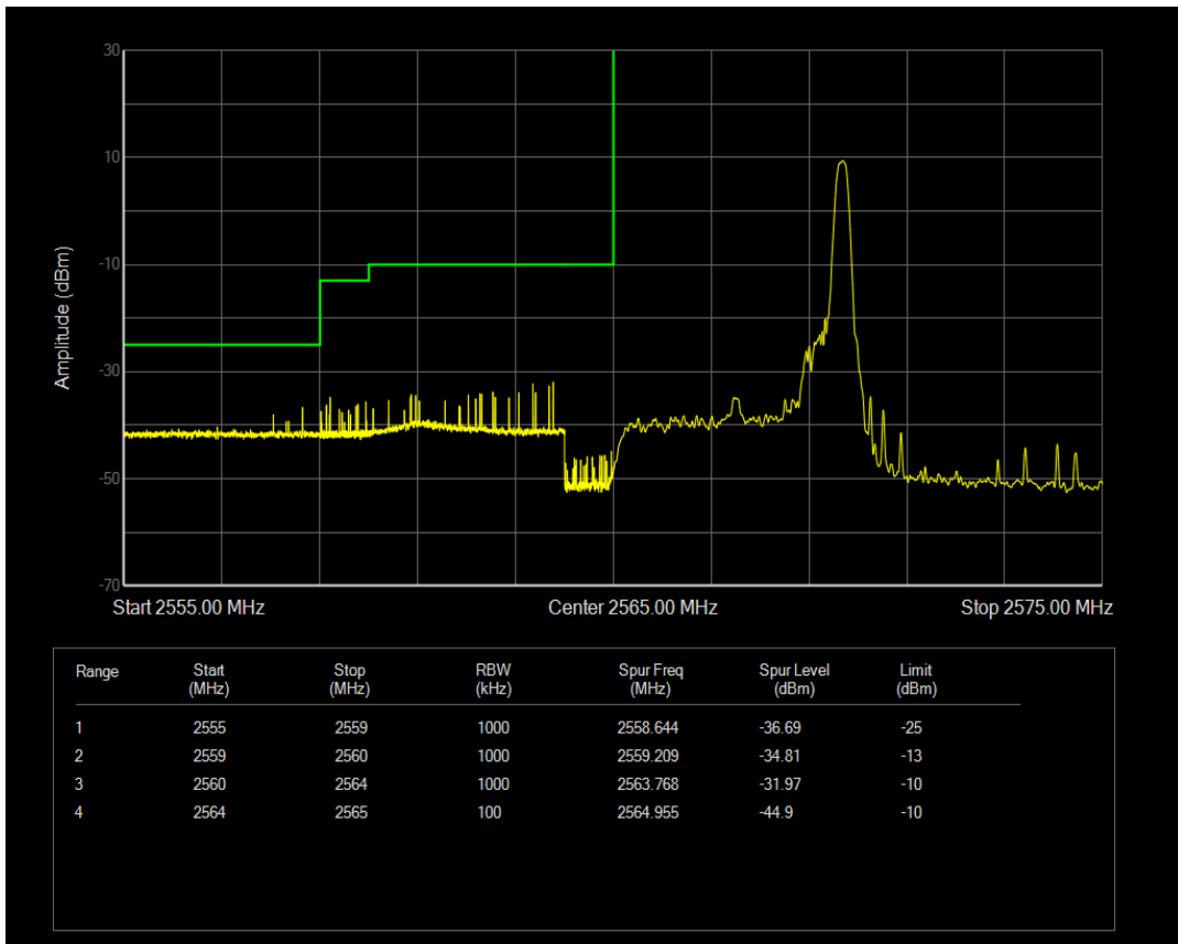
Band41 QPSK BW=5MHz Channel=40365 RB Size=25 Position=#0
