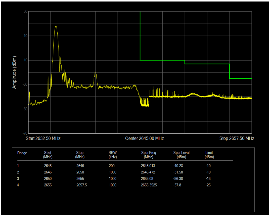
Band41 16QAM BW=10MHz Channel=41090 RB Size=1 Position=#Max
