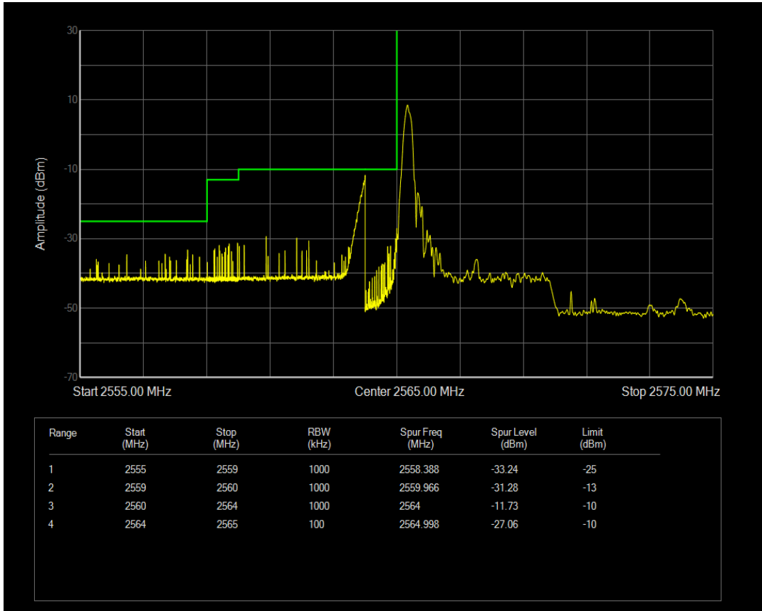
Band41 QPSK BW=5MHz Channel=40365 RB Size=1 Position=#Max
