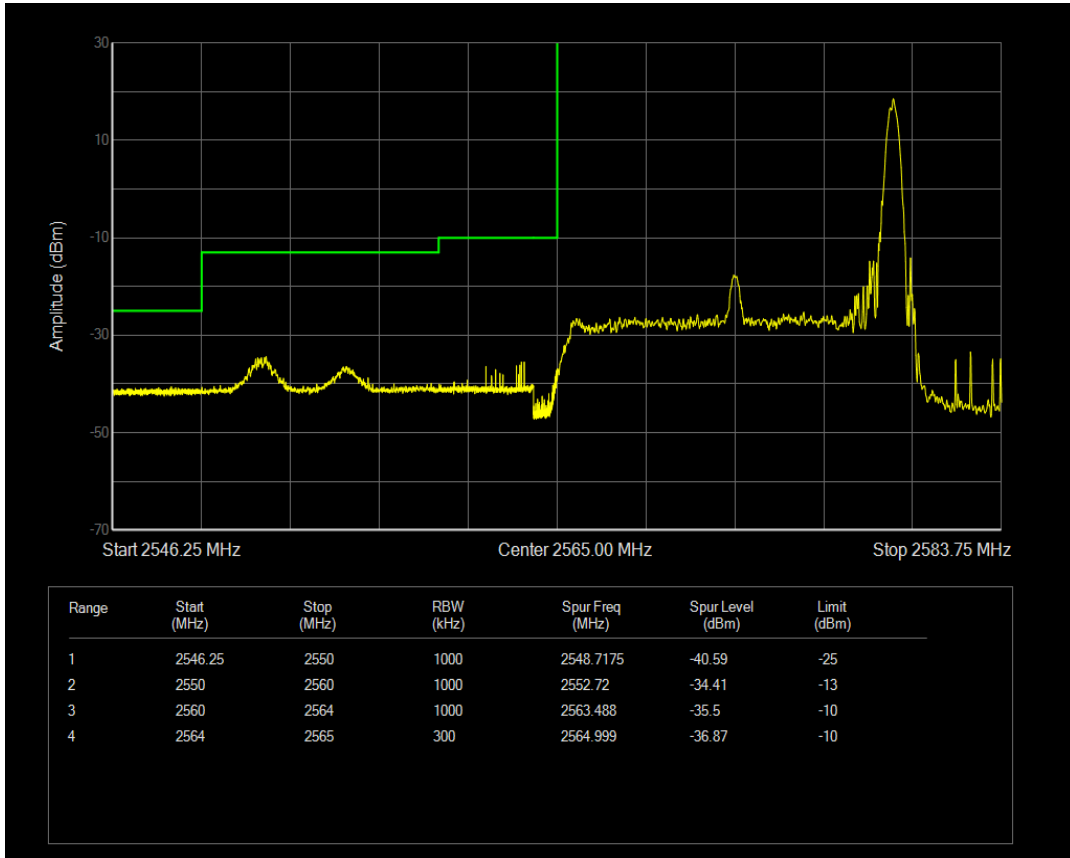
Band41 16QAM BW=15MHz Channel=40415 RB Size=75 Position=#0
