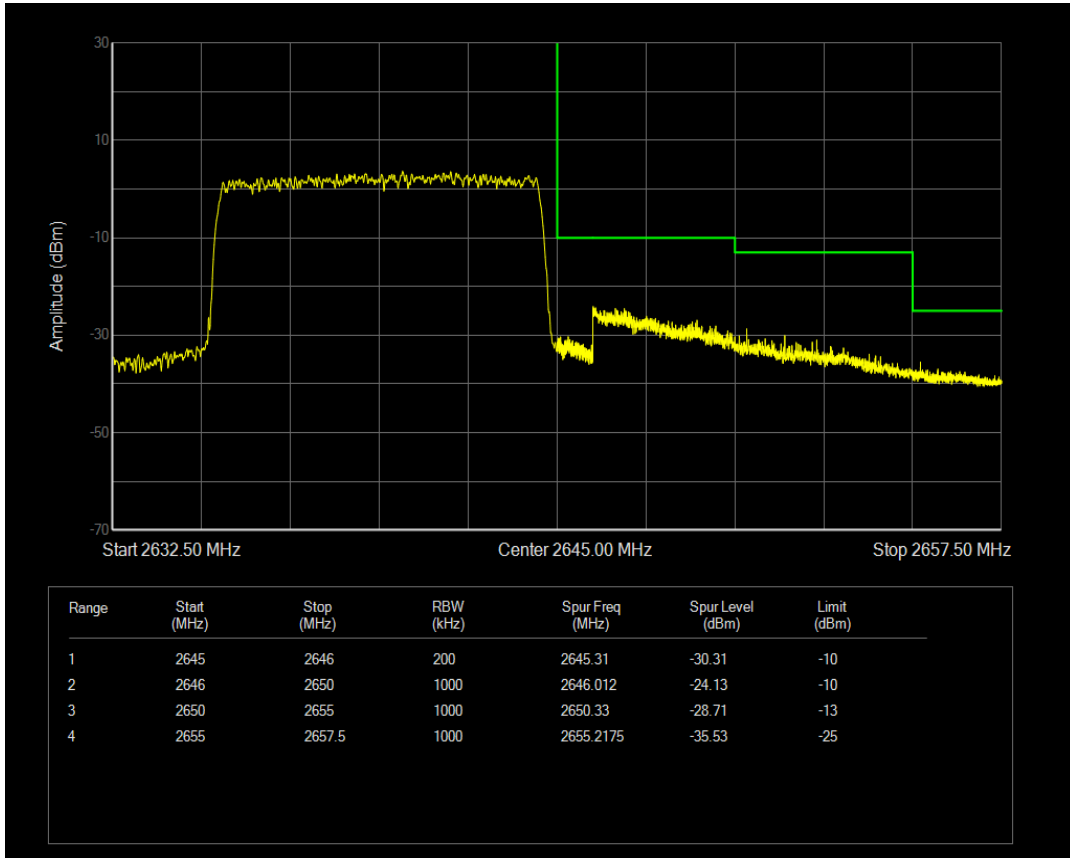
Band41 16QAM BW=10MHz Channel=41090 RB Size=1 Position=#0
