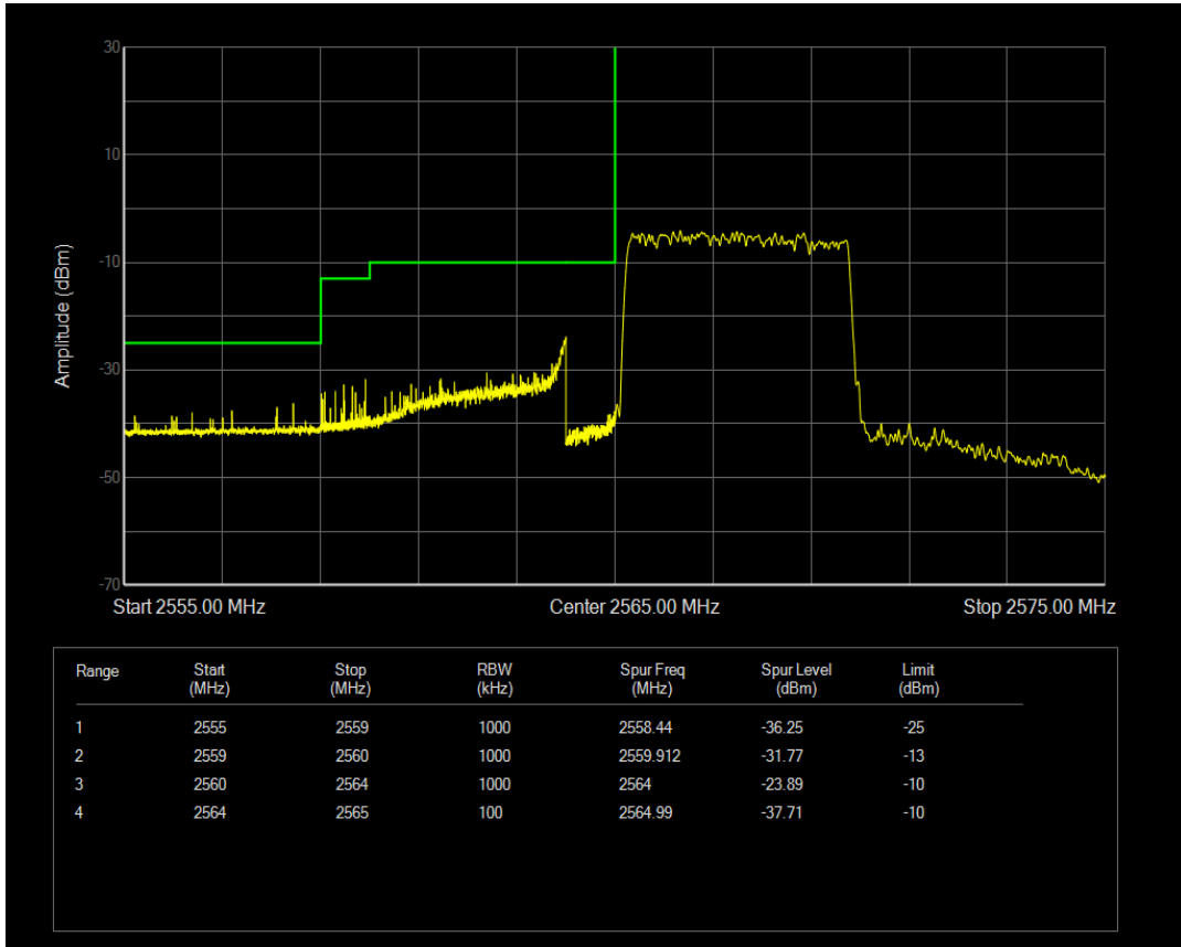
Band41 16QAM BW=5MHz Channel=40365 RB Size=1 Position=#0
