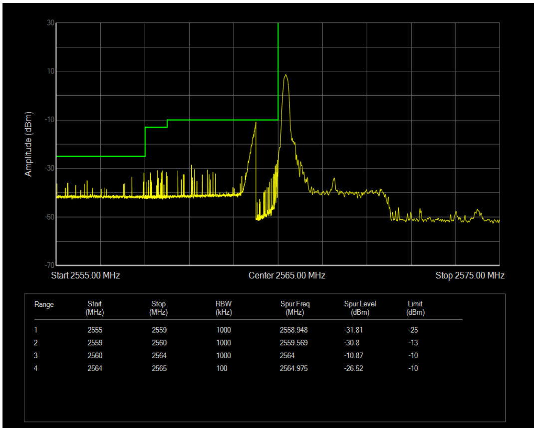
Band41 16QAM BW=5MHz Channel=40365 RB Size=1 Position=#Max
