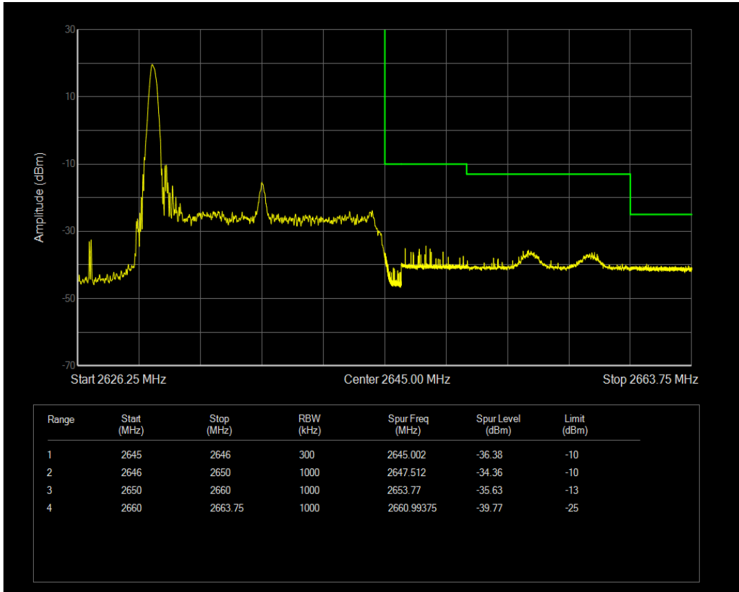
Band41 QPSK BW=15MHz Channel=41065 RB Size=1 Position=#Max
