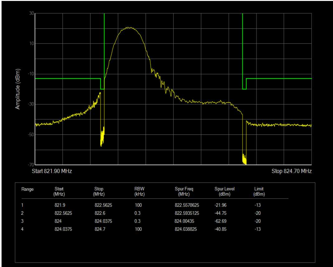
Band26(814-824) QPSK BW=1.4MHz Channel=26783 RB Size=1 Position=#Max
