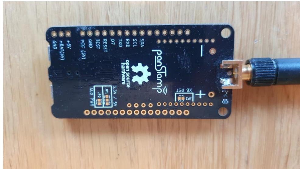
PCB Front
