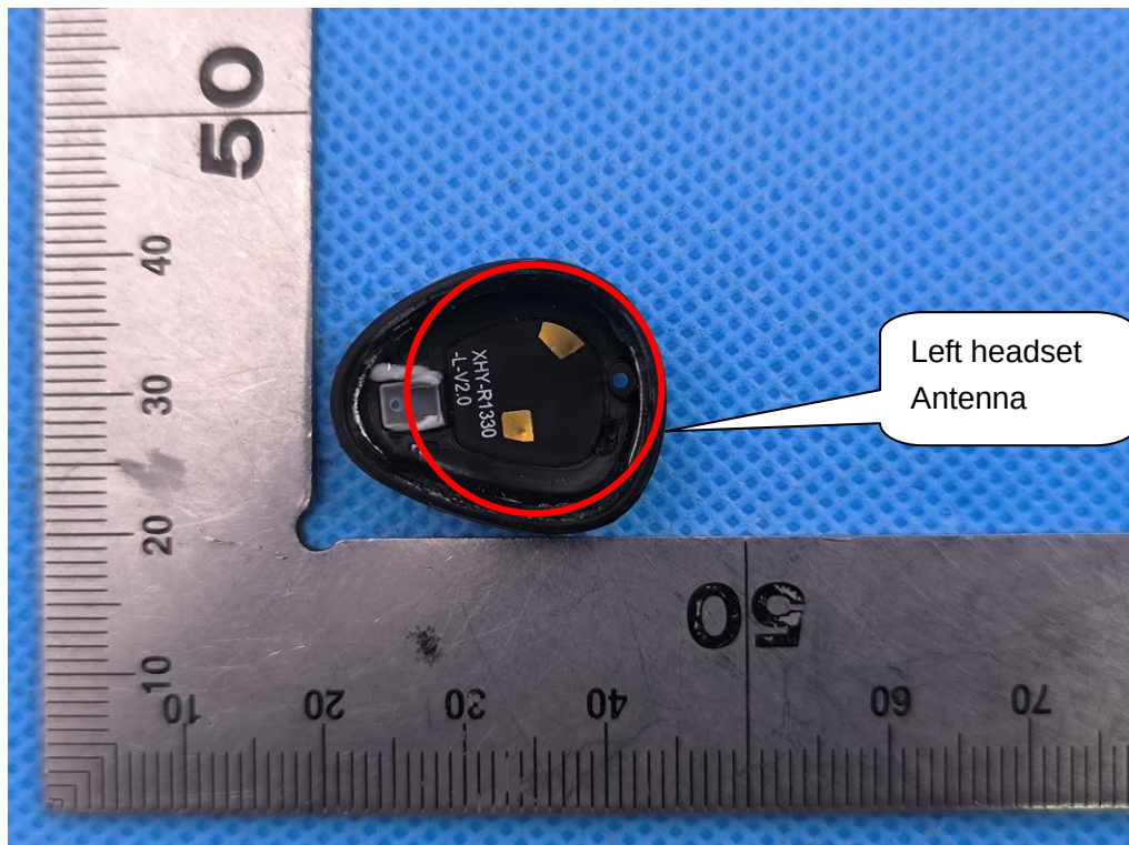
ANTENNA of EUT-1
