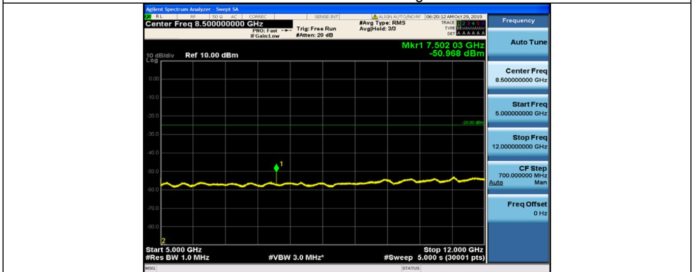
Band7-10MHz-16QAM-20800-1RB#0-Range3:5000~12000MHz
