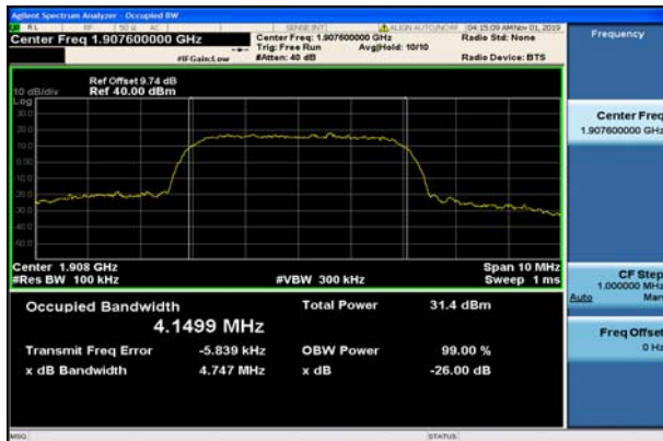
WCDMA Band II – 1907.6MHz
