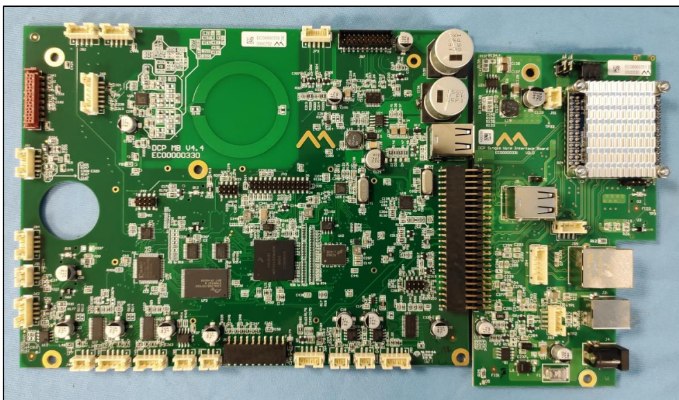
Main Board and Interface Board - Top view
