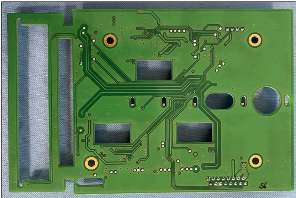
Dual feeder Control Board - Bottom view
