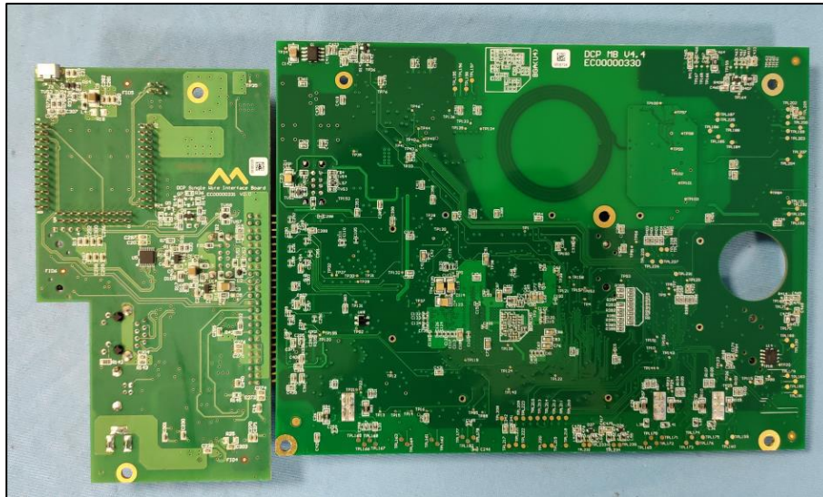
Main Board and Interface Board - Bottom view
