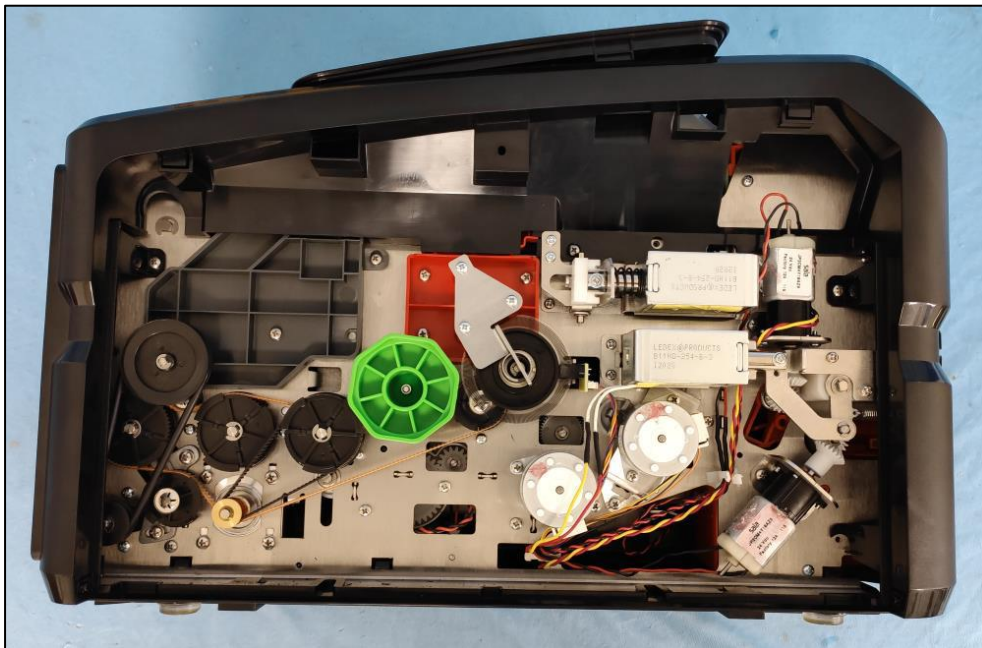
Internal Construction – Side view
