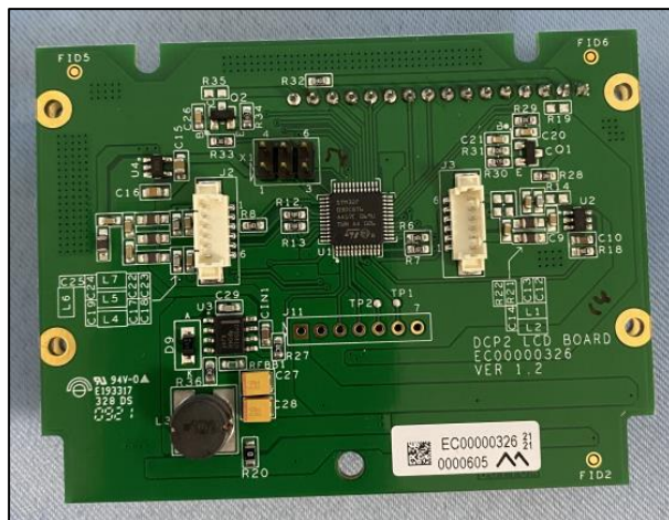
LCD Board - Bottom view
