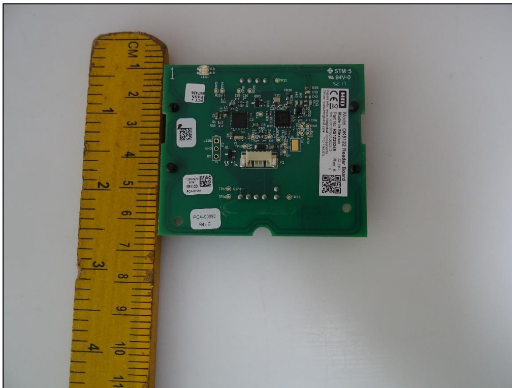
HID_PCB_Dimensional View
