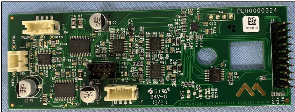
Magnetic Encoder Board - Top view
