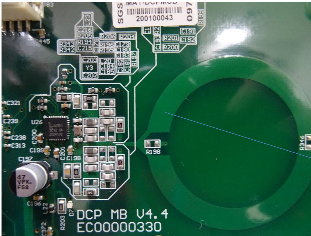
MC310 Printer main board RFID Section
