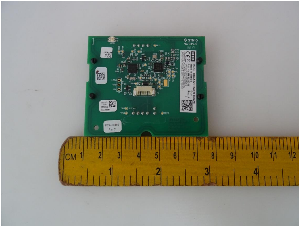
HID RFID board dimensional view (Width)
