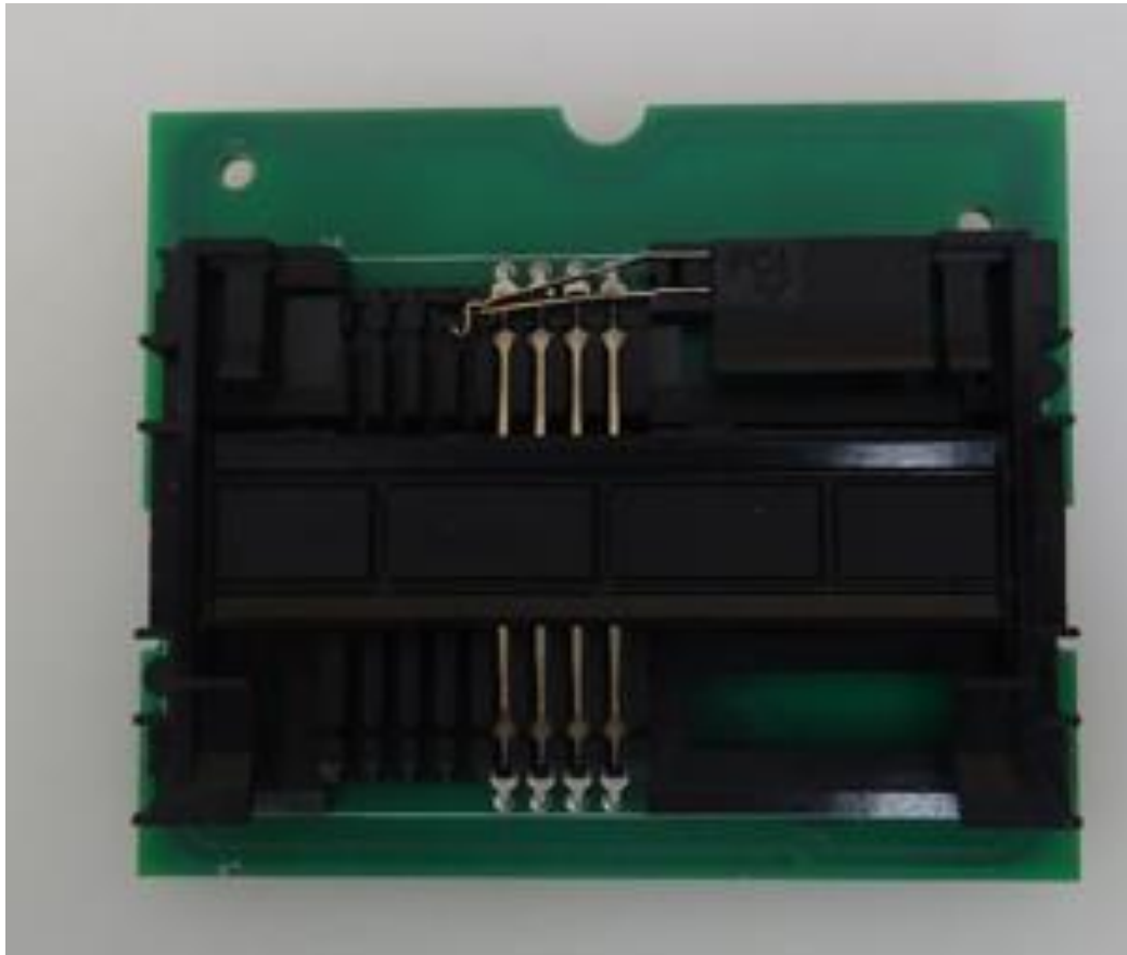
HID RFID board Rear view
