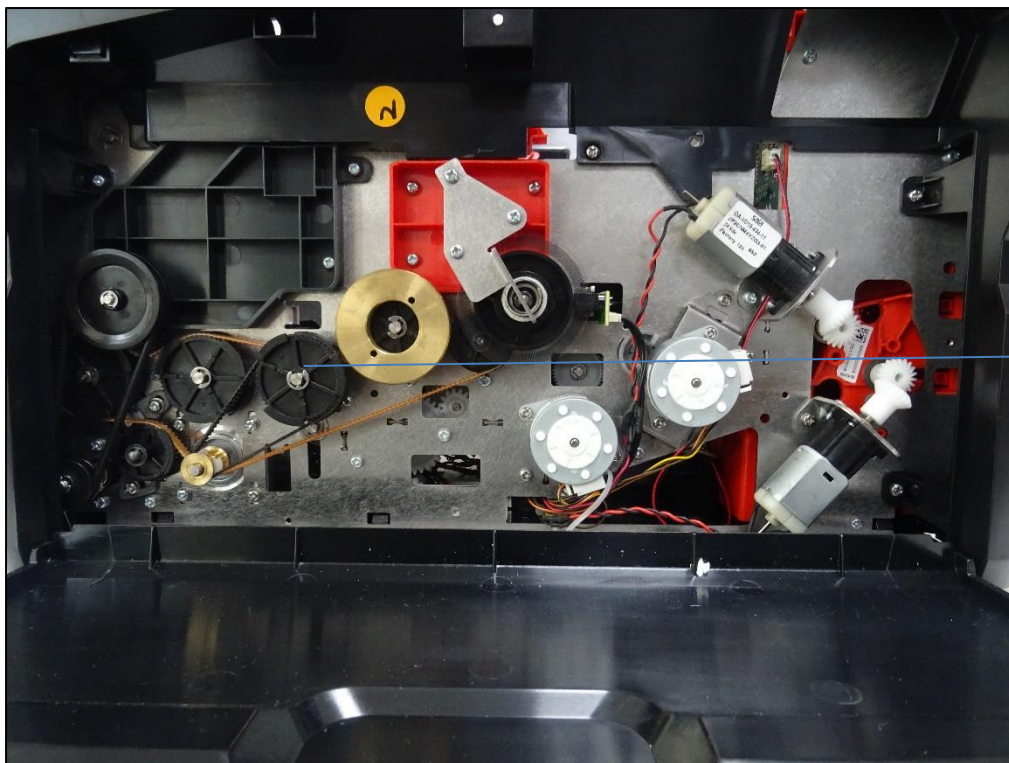
MC310 printer Mechanical section view
