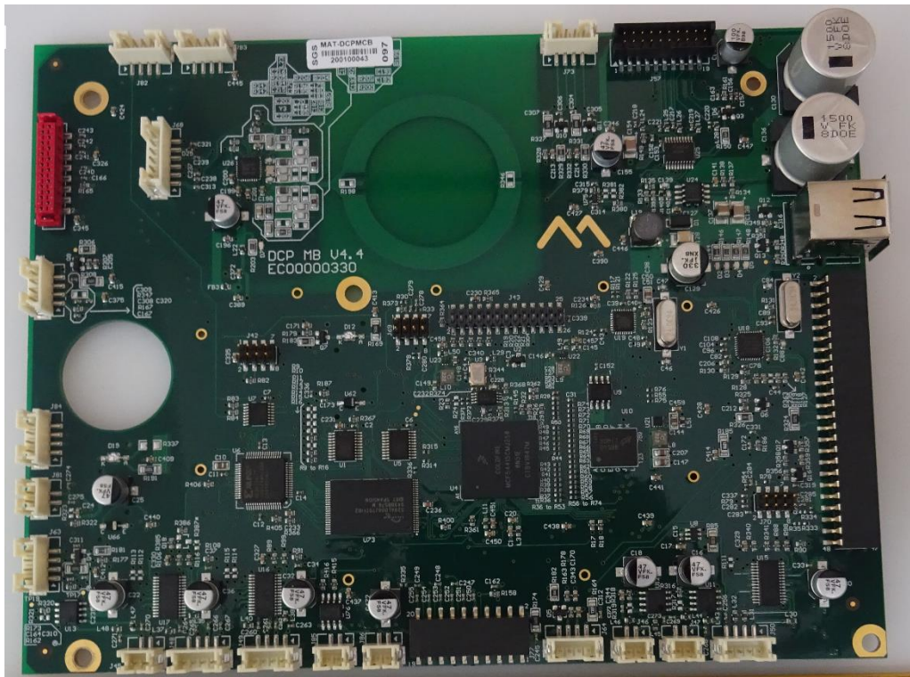
MC310 Printer main board front view
