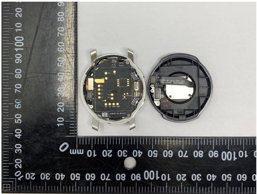
Fig. 2. Internal view-01
