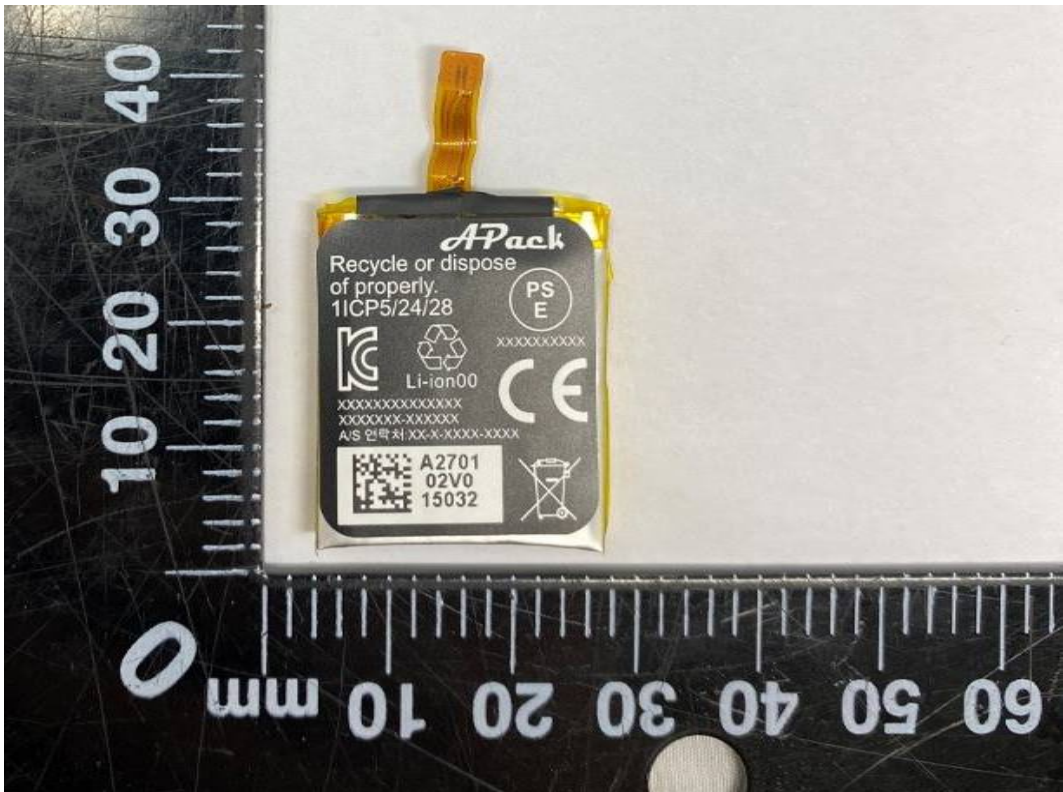
Fig. 7. Battery view-02
