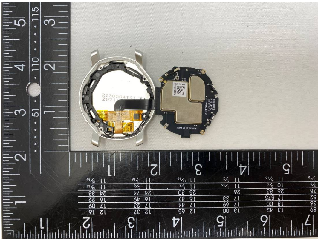
Fig. 4. PCB view-01
