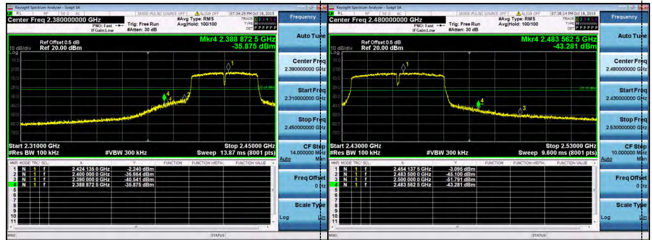
Left bandedge
