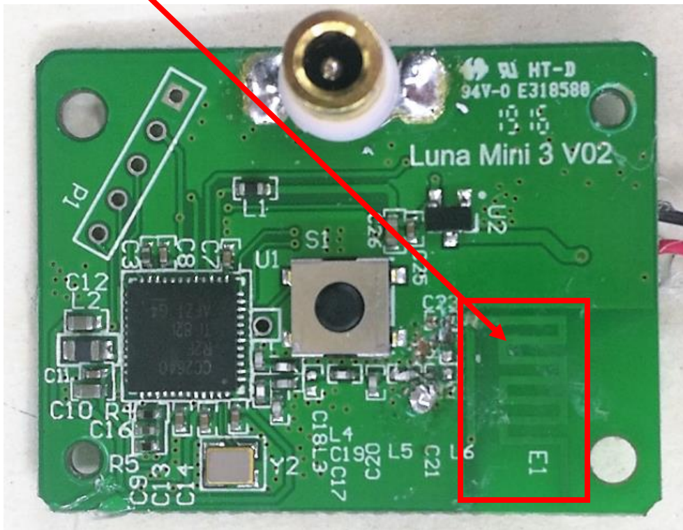
Antenna location
