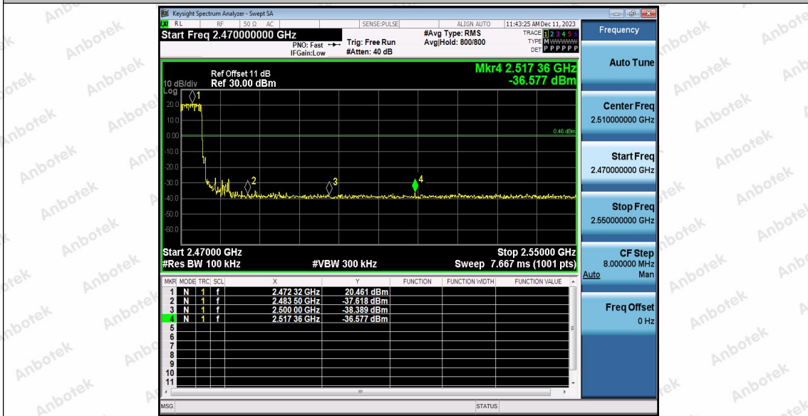
2.4G_Ant1_High_Hop_2474.1
