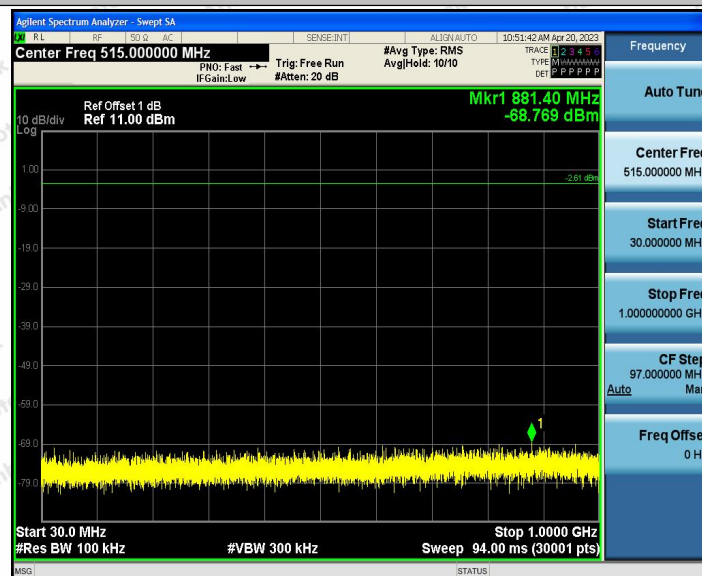
2.4G_Ant1_2440.9_30~1000
