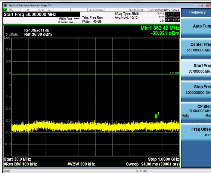
2.4G_Ant1_2440.8_30~1000
